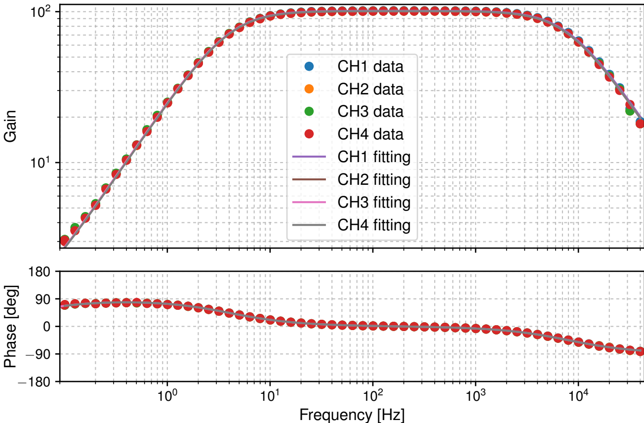
Transfer function AC
