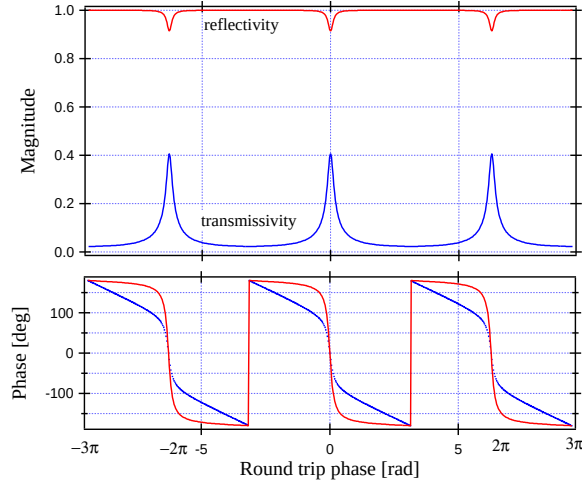
Figure 1.5: Response of a Fabry-Perot cavity. The optical parameters of the mirror were chosen arbitrarily to obtain clear view.
