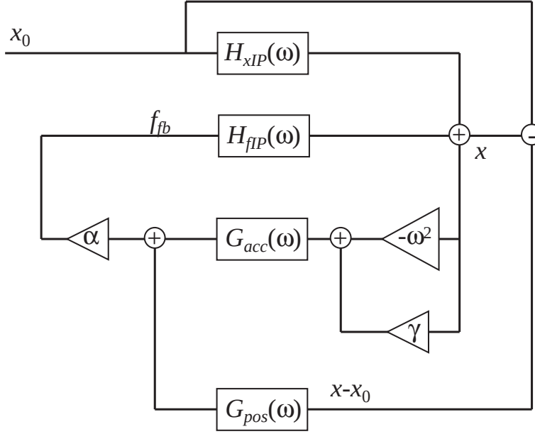
Figure 6.6: Block diagram of the asymmetric IP control.
