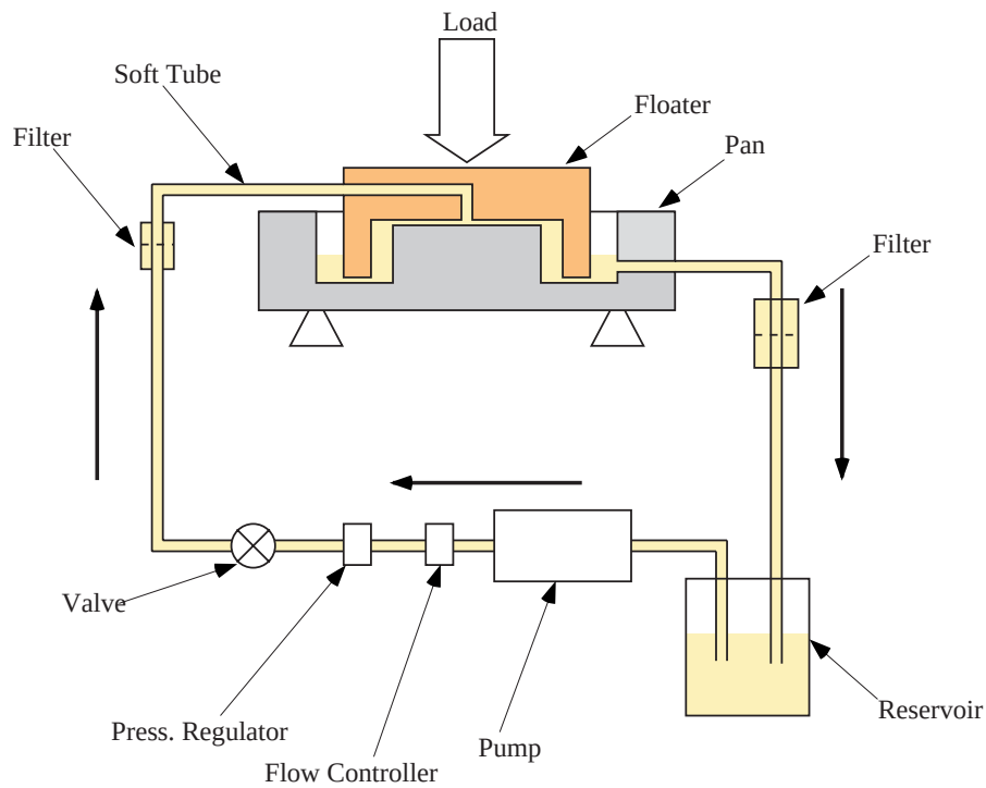
Figure 2.15: The oil bearing system. The oil is driven by a pump, and the flow and the pressure is controlled by regulators. Also there are two sieve filters in the path to remove residual dusts from the circulation. Tubes in the path is all made of flexible polyvinyl chloride that doesn't constrain free motion of moving parts. The load is applied on a floater made of brass, and there is an oil channel oil in the floater, opening downwards at the center. The oil flows through the channel into an oil pan, forming a thin film which greatly reduces the friction between the floater and the pan.
