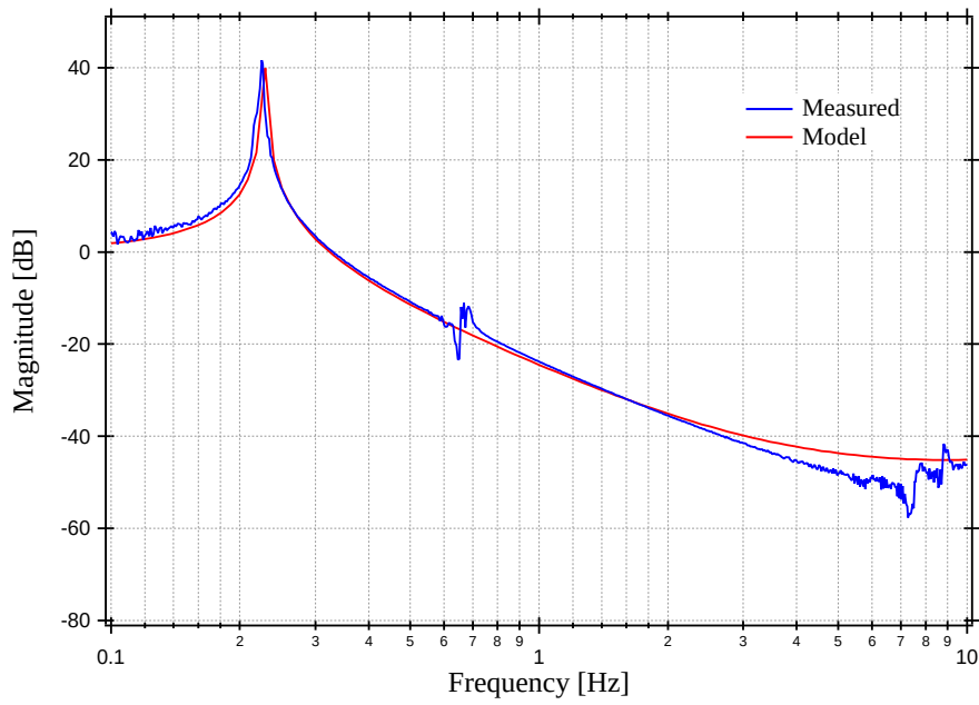
Figure 2.17: Horizontal transfer function of the prototype IP, tuned at 220 mHz. Structure around 650 mHz is caused by cross-coupling from the rotational mode of the IP. The plateau level given at 10 Hz is -47 dB.
