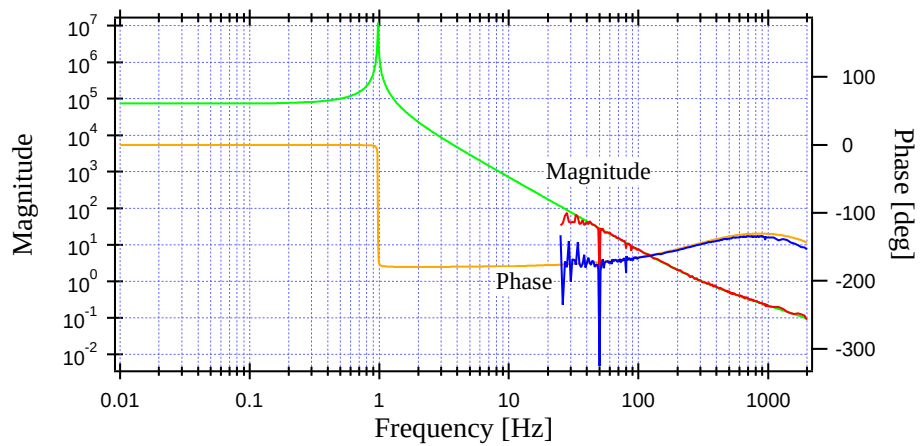
Figure 7.7: Open loop transfer function of the cavity control. Measured (Red, Blue) and Fitted (Green, Yellow)
