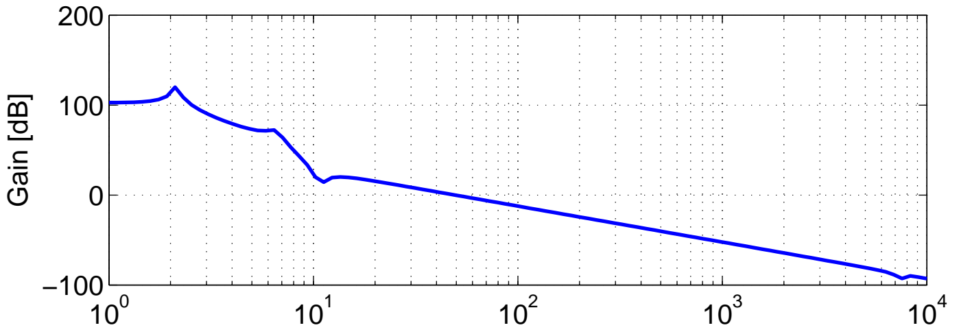
SRCL Raw Gain (without feedback filter)
