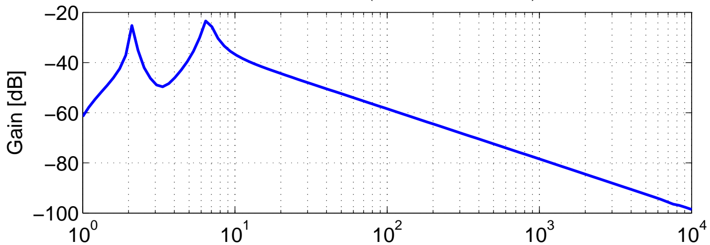
CARM Raw Gain (without feedback filter)
