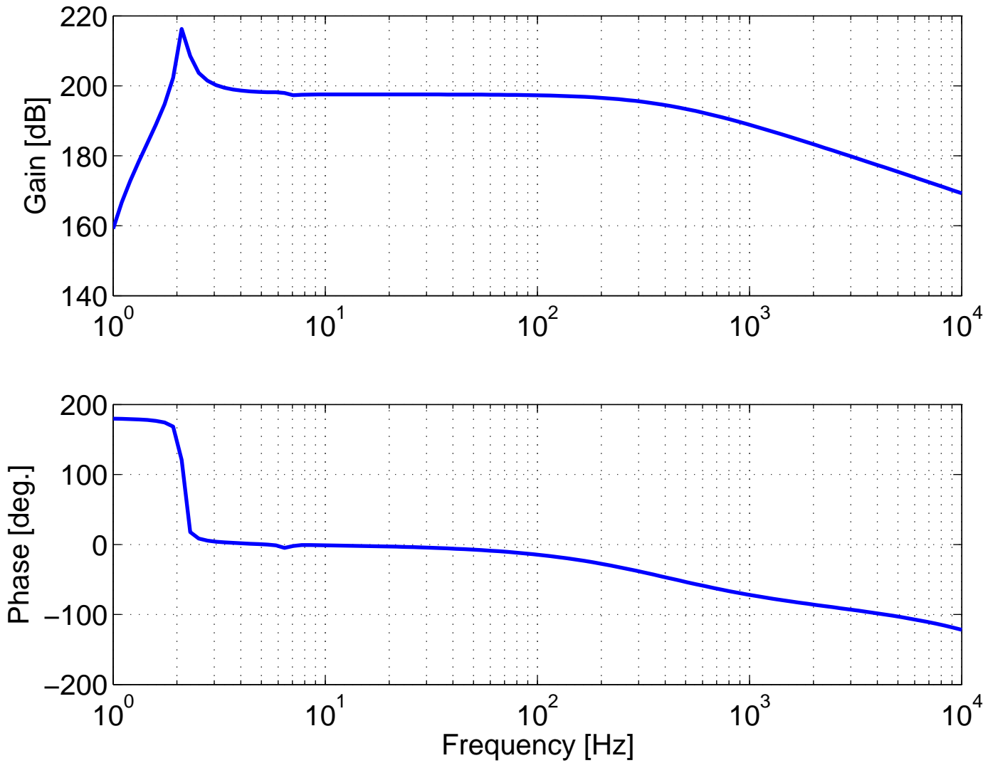
DARM Optical Gain
