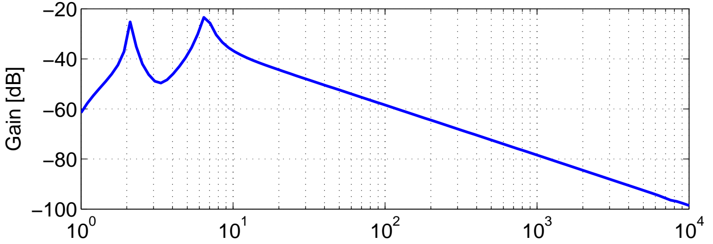
CARM Optical Gain
