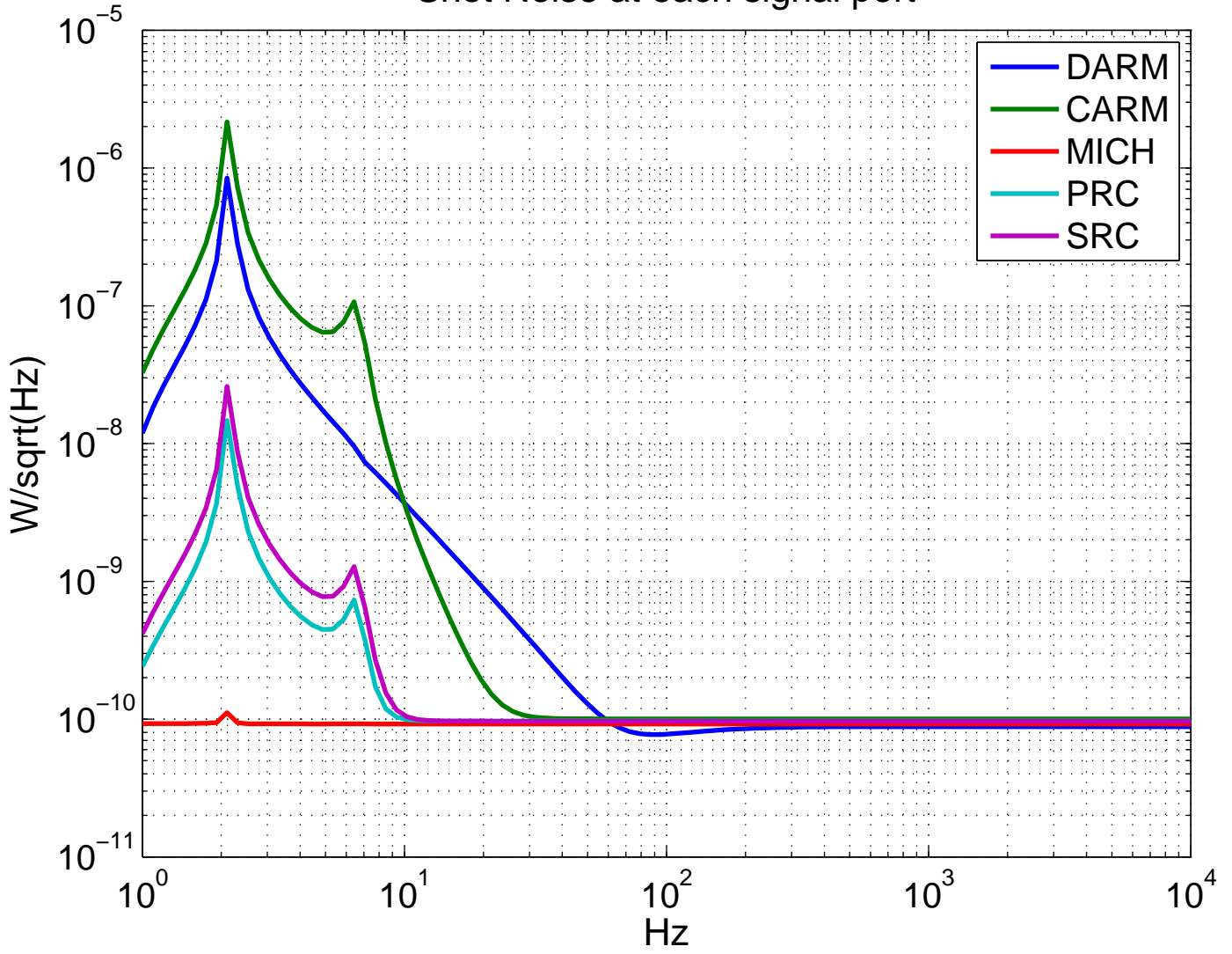
Shot Noise at each signal port
