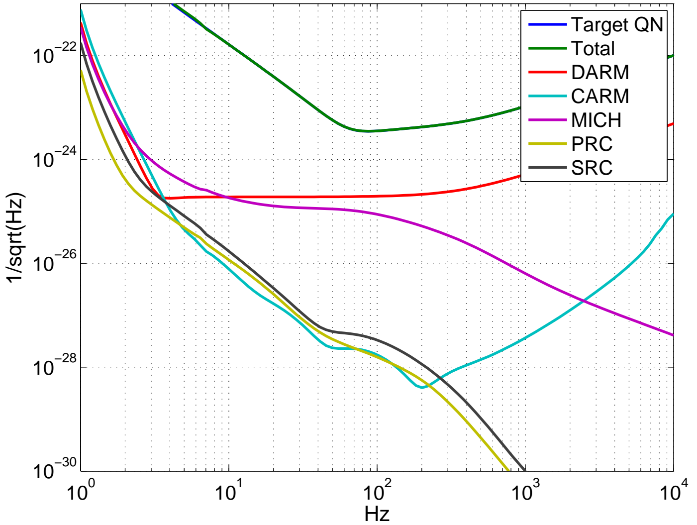
PD Noise Coupling with Feed Forward
