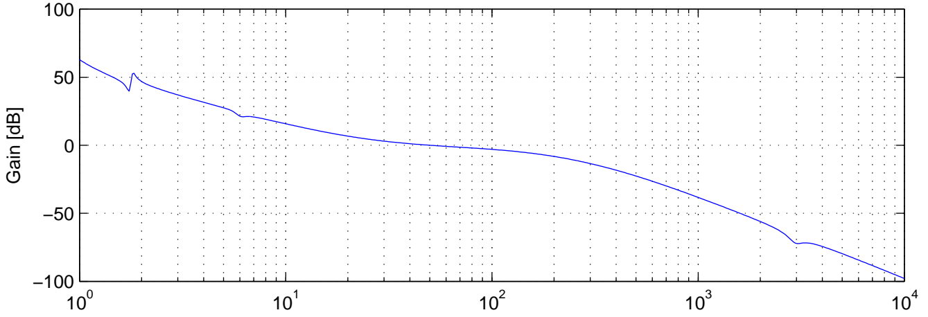
PRC Open Loop Gain
