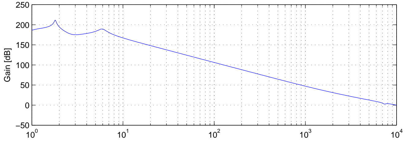
CARM Open Loop Gain
