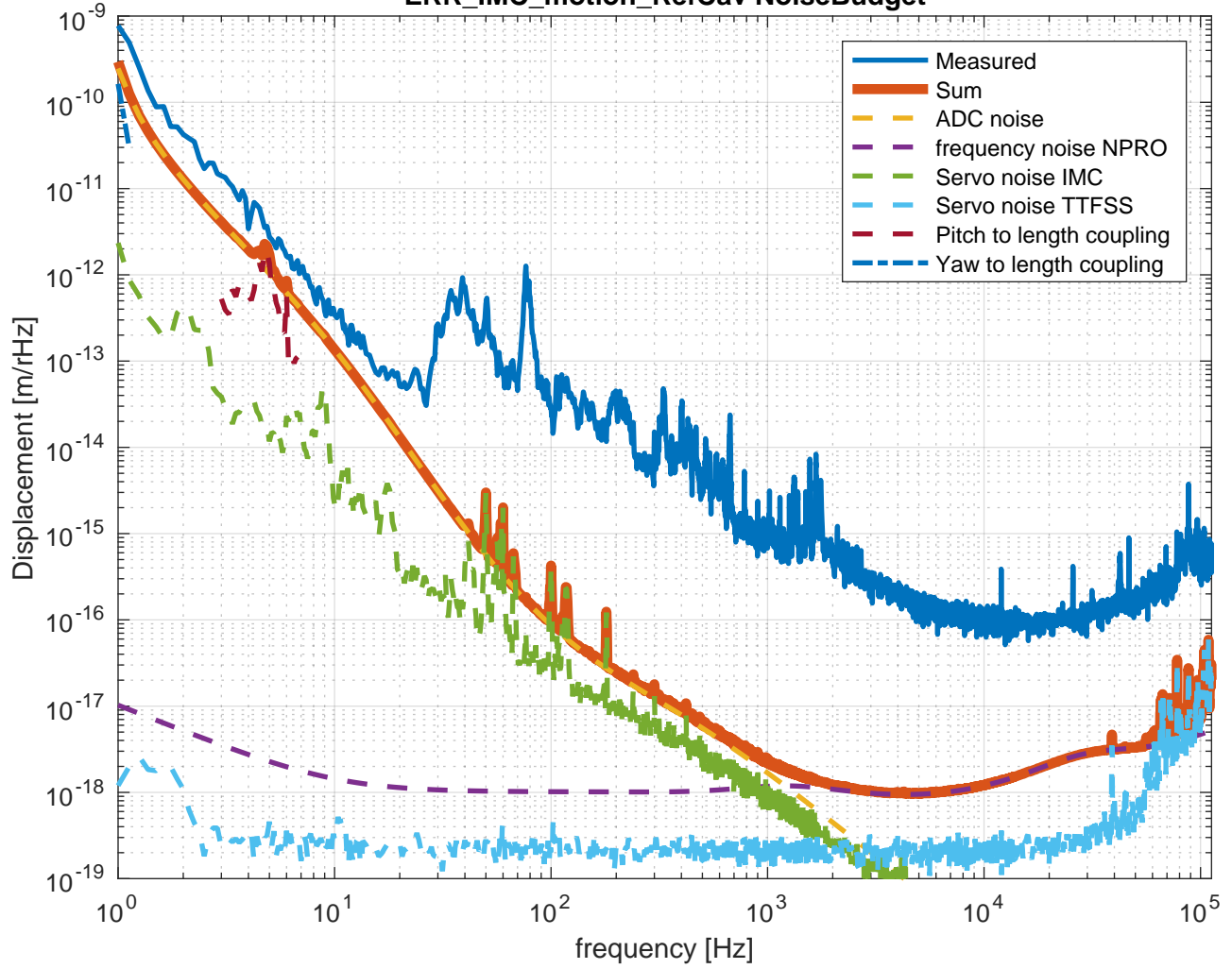
ERR_IMC_motion_RefCav NoiseBudget
