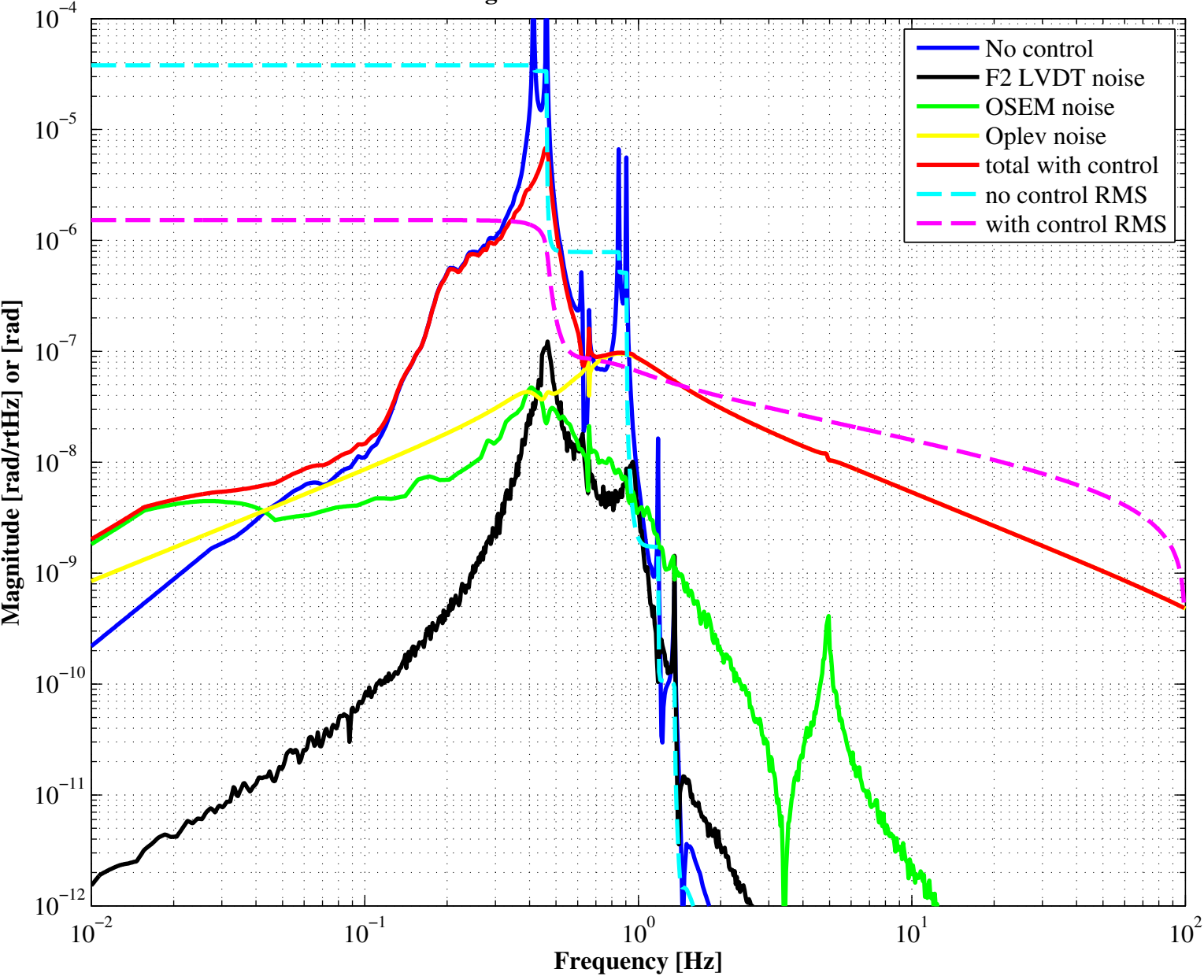
Angular Fluctuation of the Mirror
