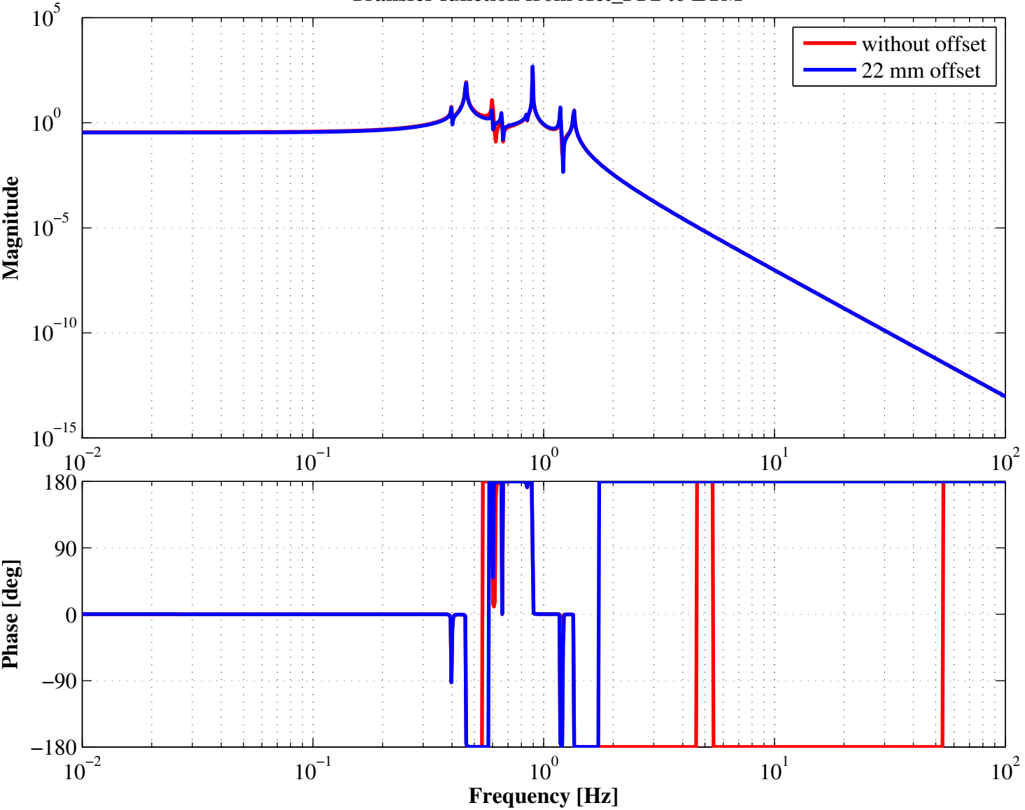
Transfer function from Act_PF2 to LTM
