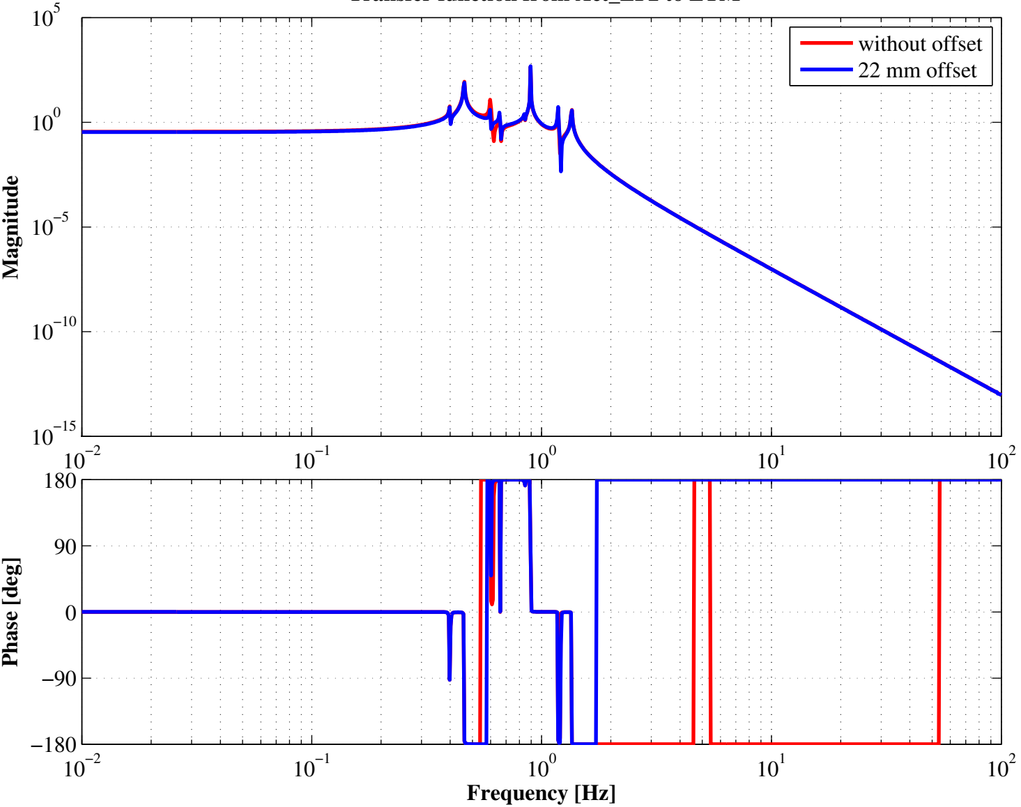
Transfer function from Act_LF2 to LTM
