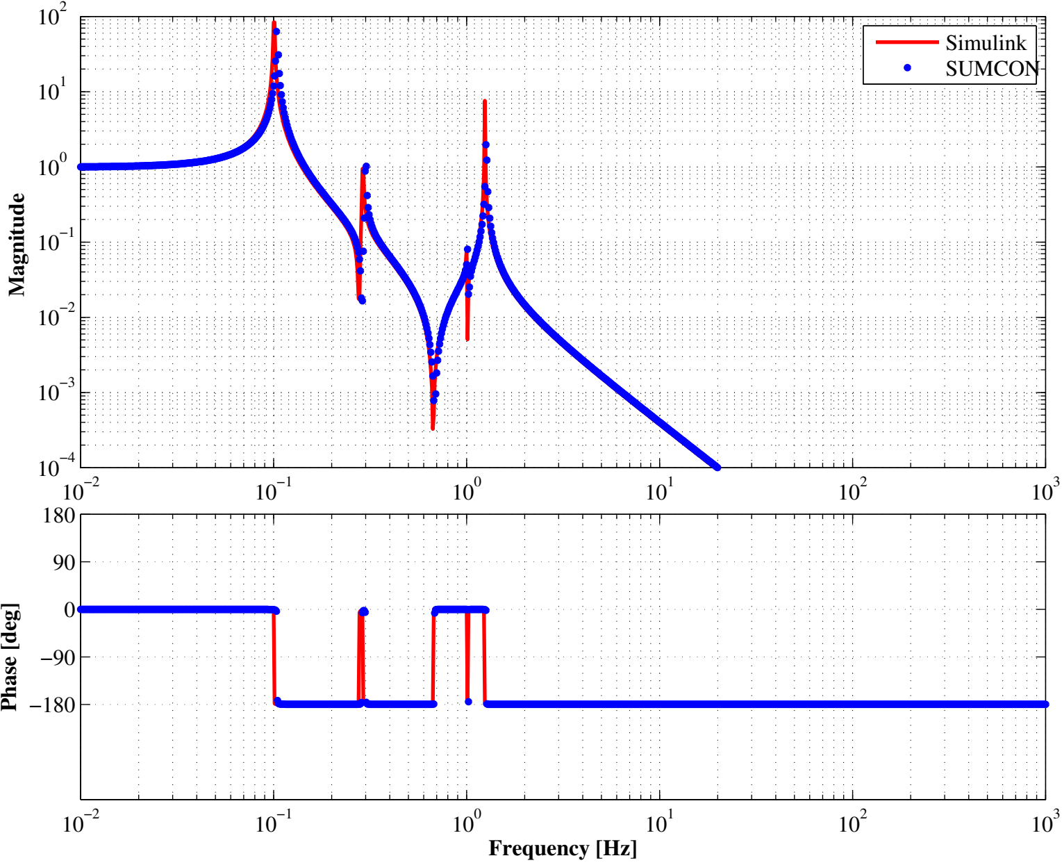
Transfer function from actYF2 to YF2
