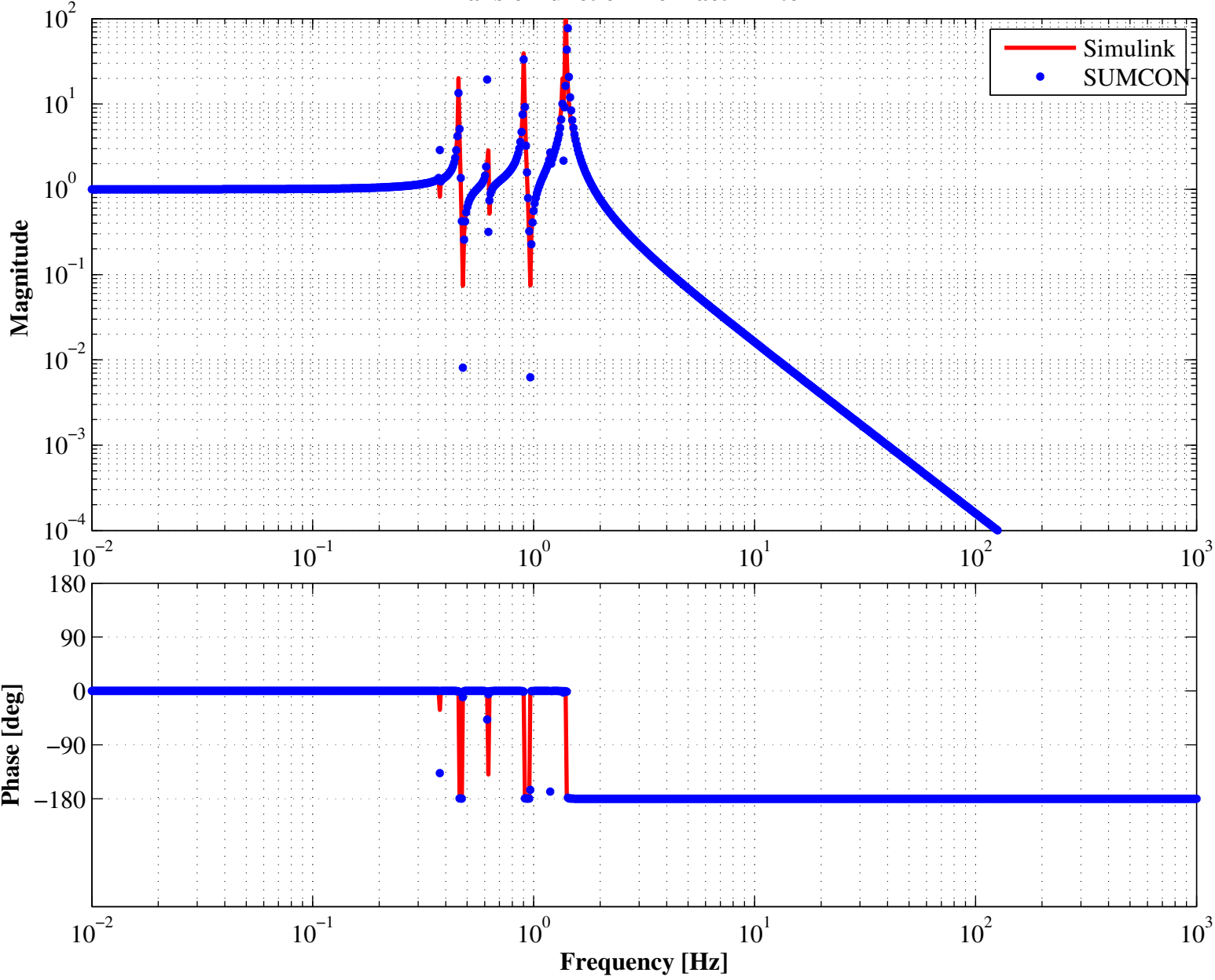
Transfer function from actTF2 to TF2
