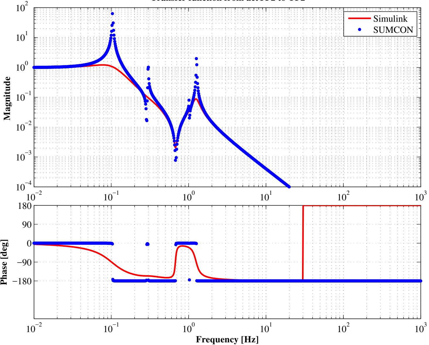
Transfer function from actYF2 to YF2
