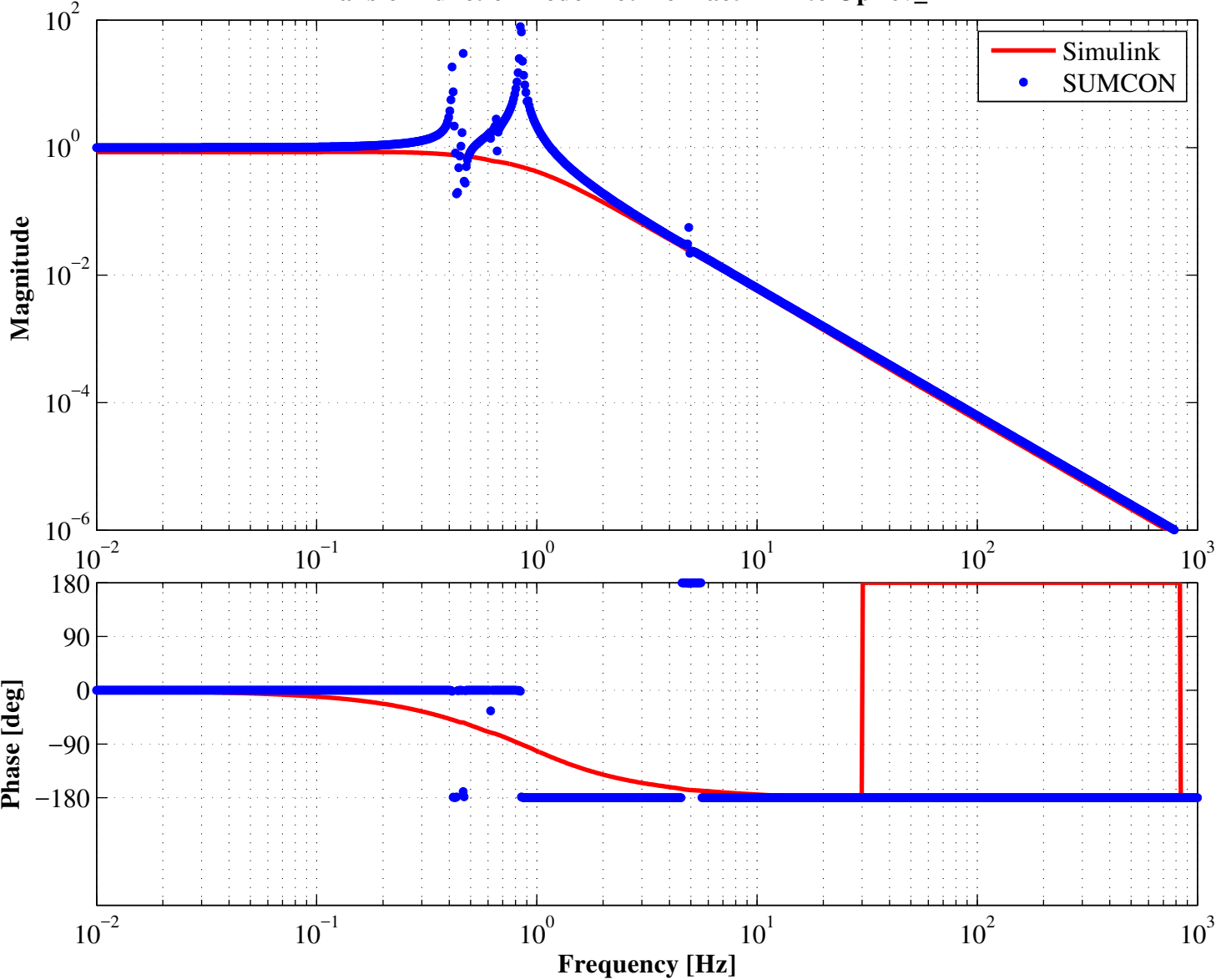
Transfer Function Bode Plot from actPTM to OpLev_PTM
