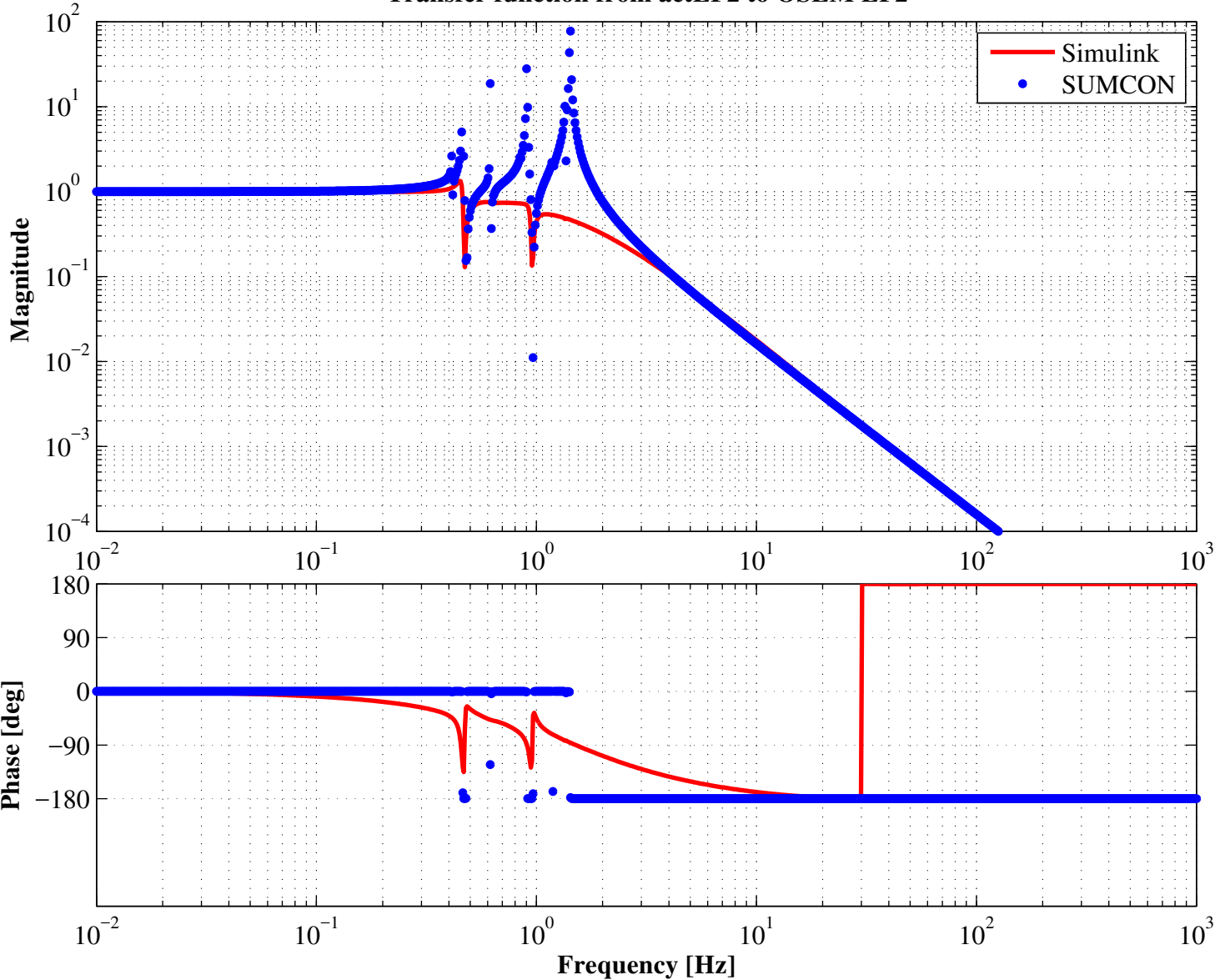
Transfer function from actLF2 to OSEM LF2
