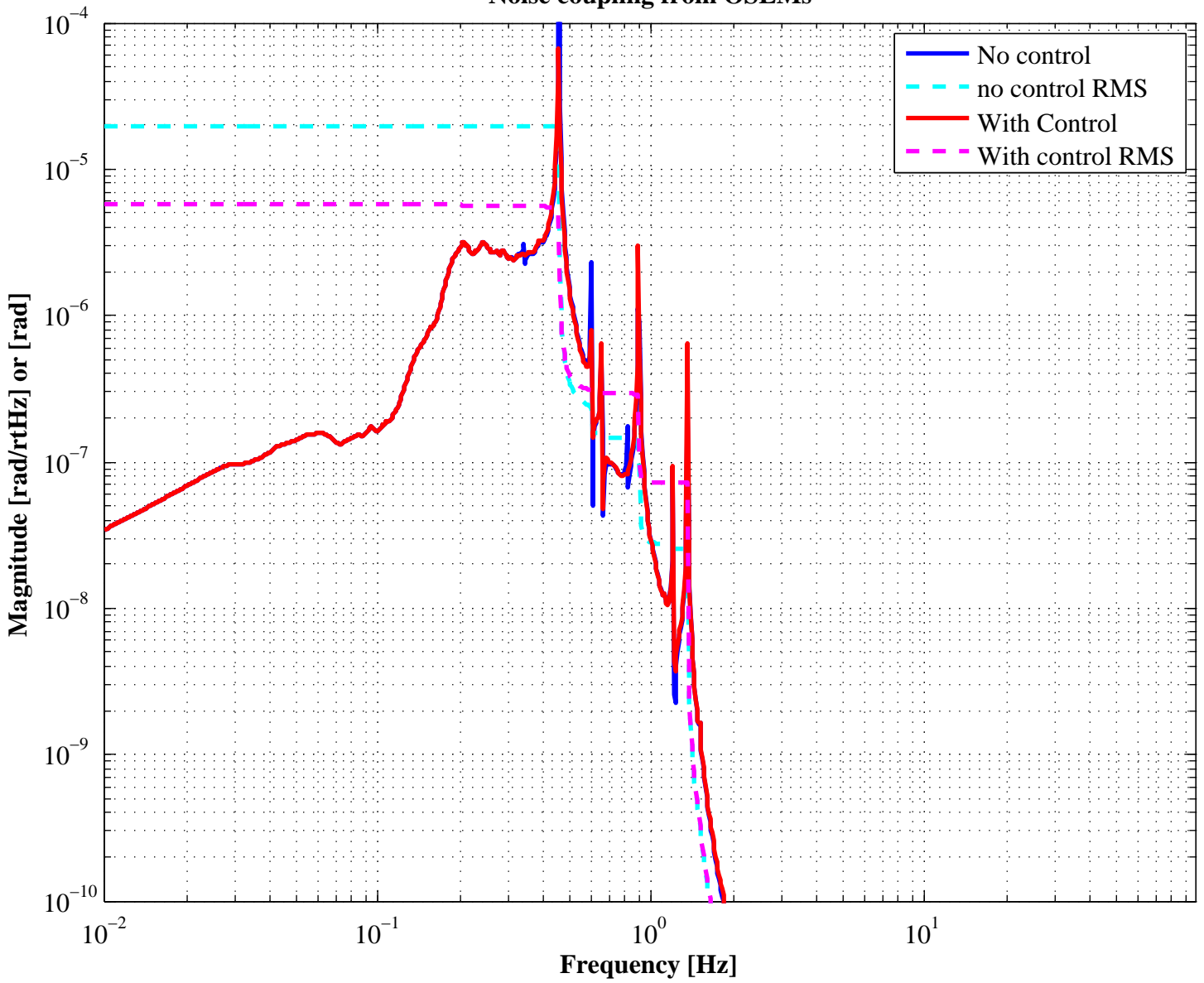
Noise coupling from OSEMs
