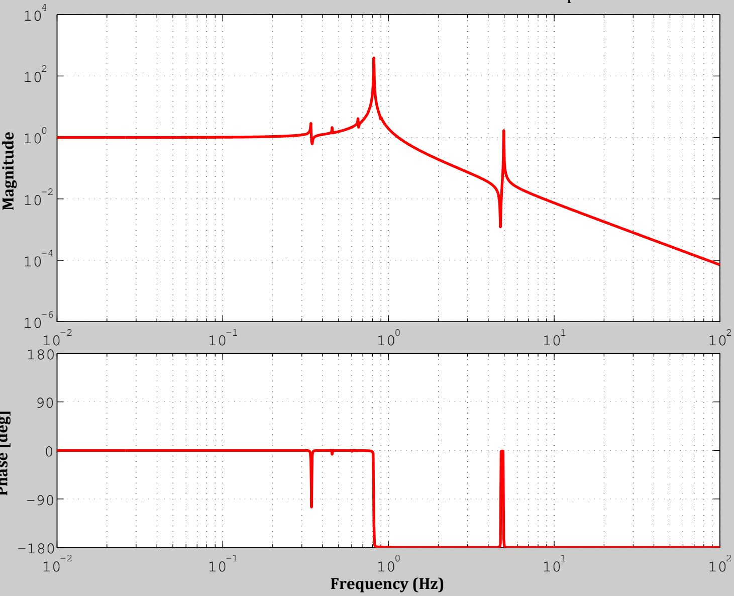
Transfer Function Bode Plot from actPTM to OSEM P TM
