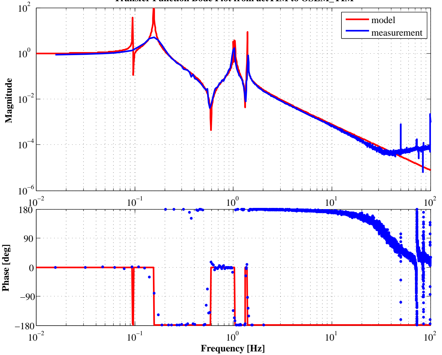
Transfer Function Bode Plot from actYIM to OSEM_YIM
