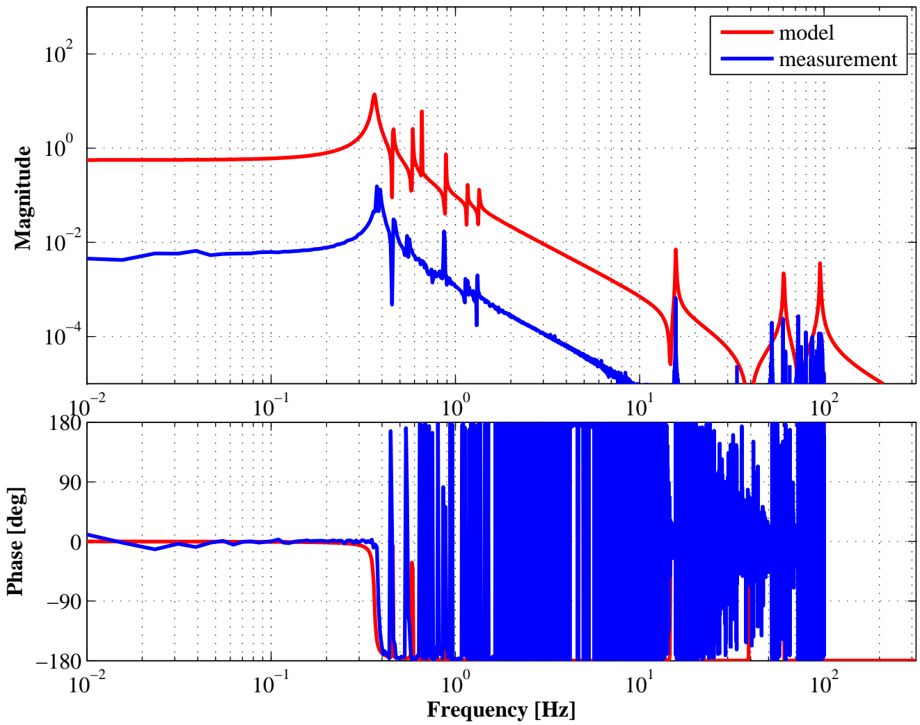
Transfer function from RIM actuator to RIM sensor
