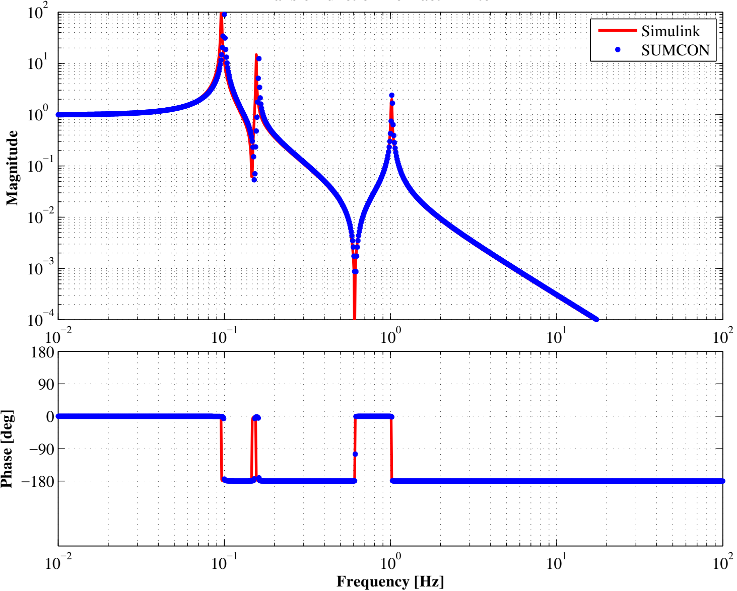
Transfer function from actYBF to YBF
