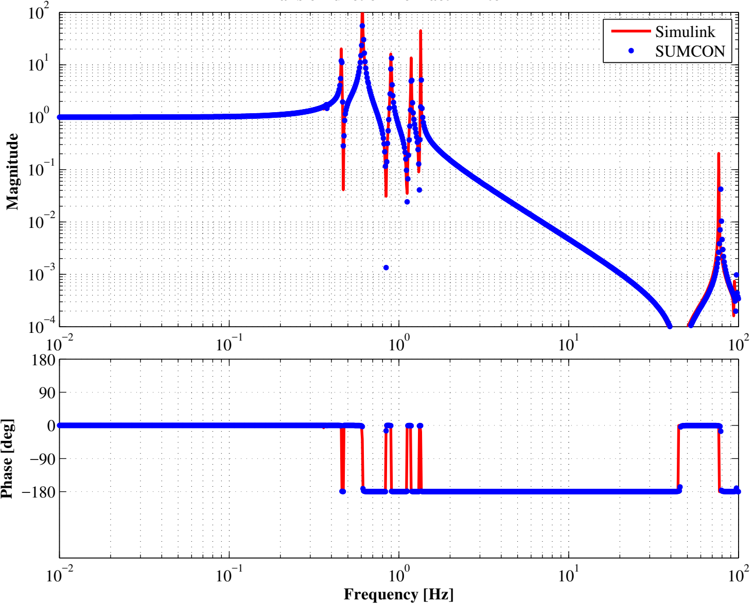
Transfer function from actRBF to RBF
