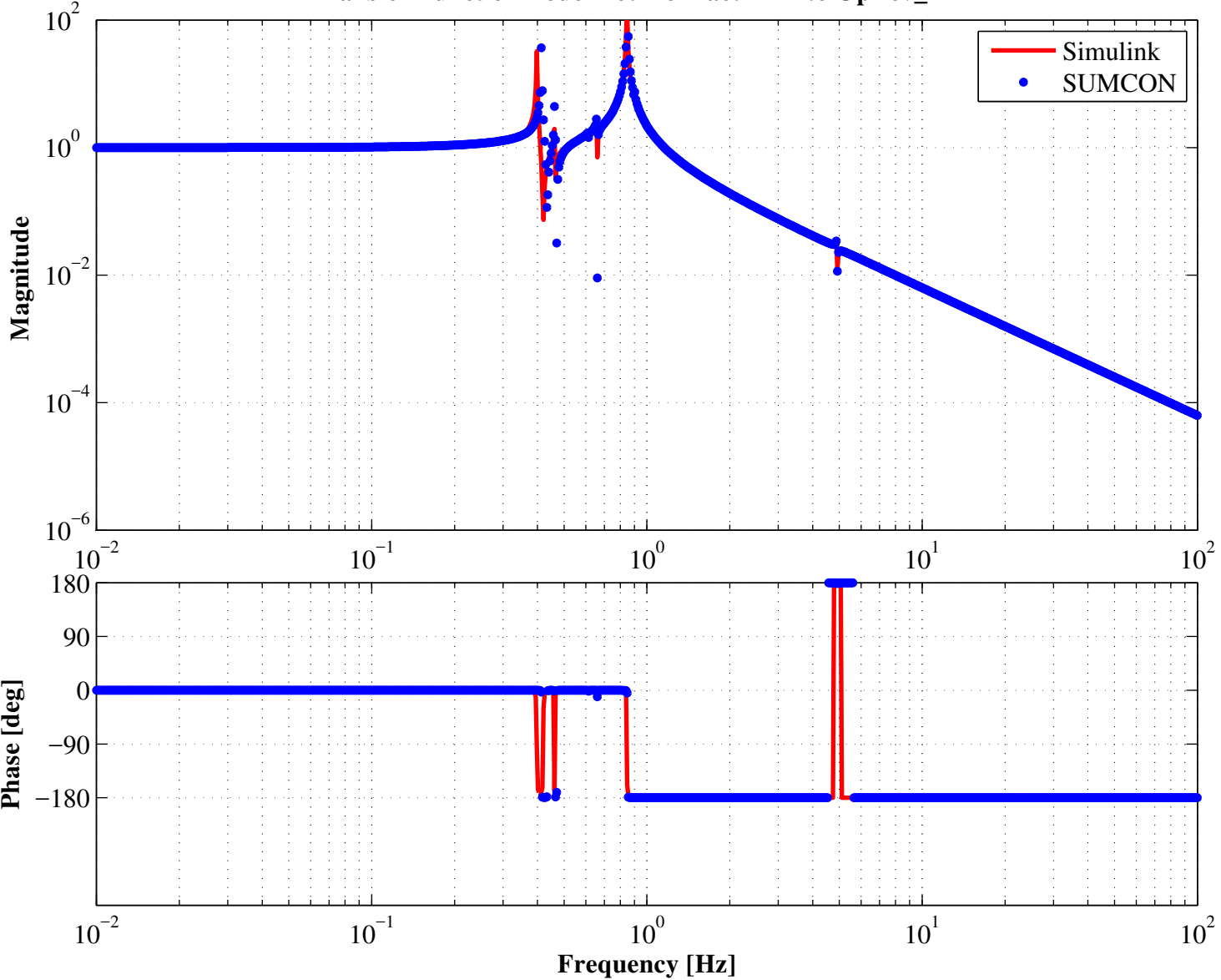
Transfer Function Bode Plot from actPTM to OpLev_PTМ
