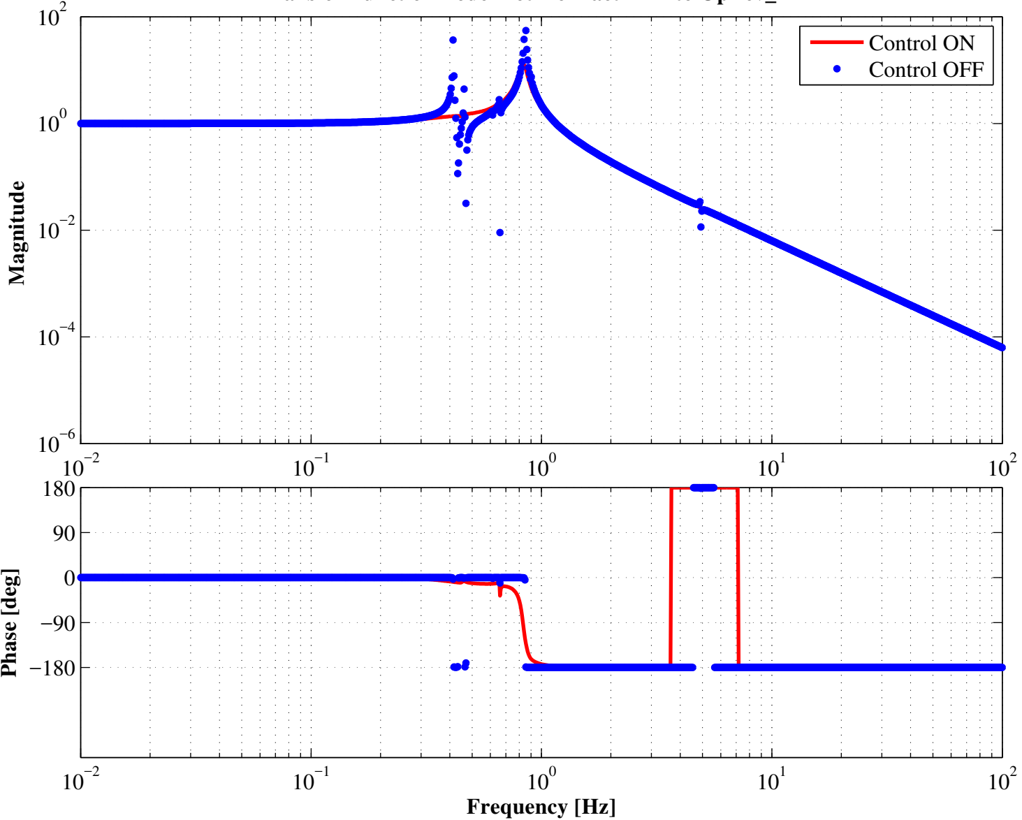
Transfer Function Bode Plot from actPTM to OpLev_PTMT
