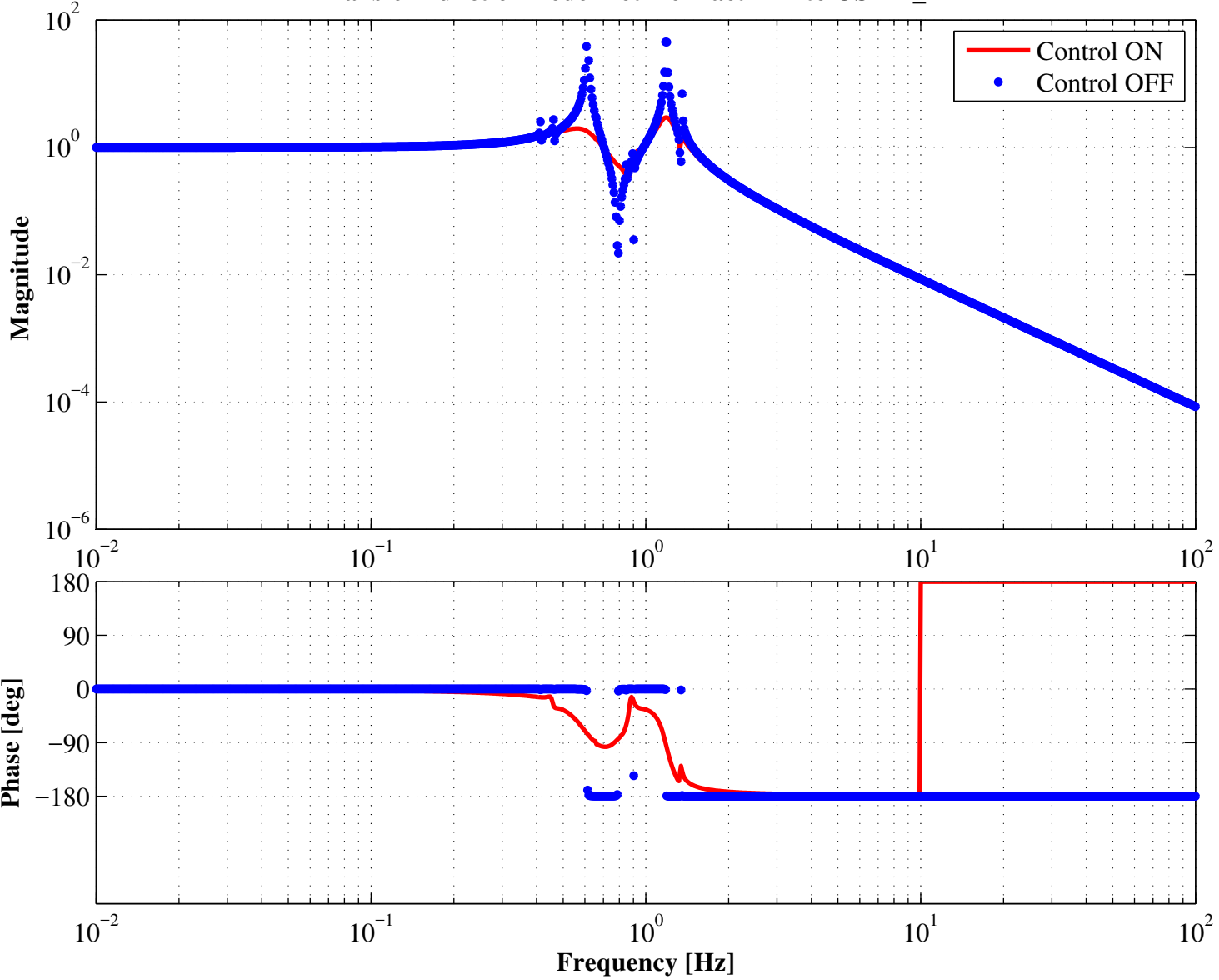
Transfer Function Bode Plot from actLIM to OSEM_LIM
