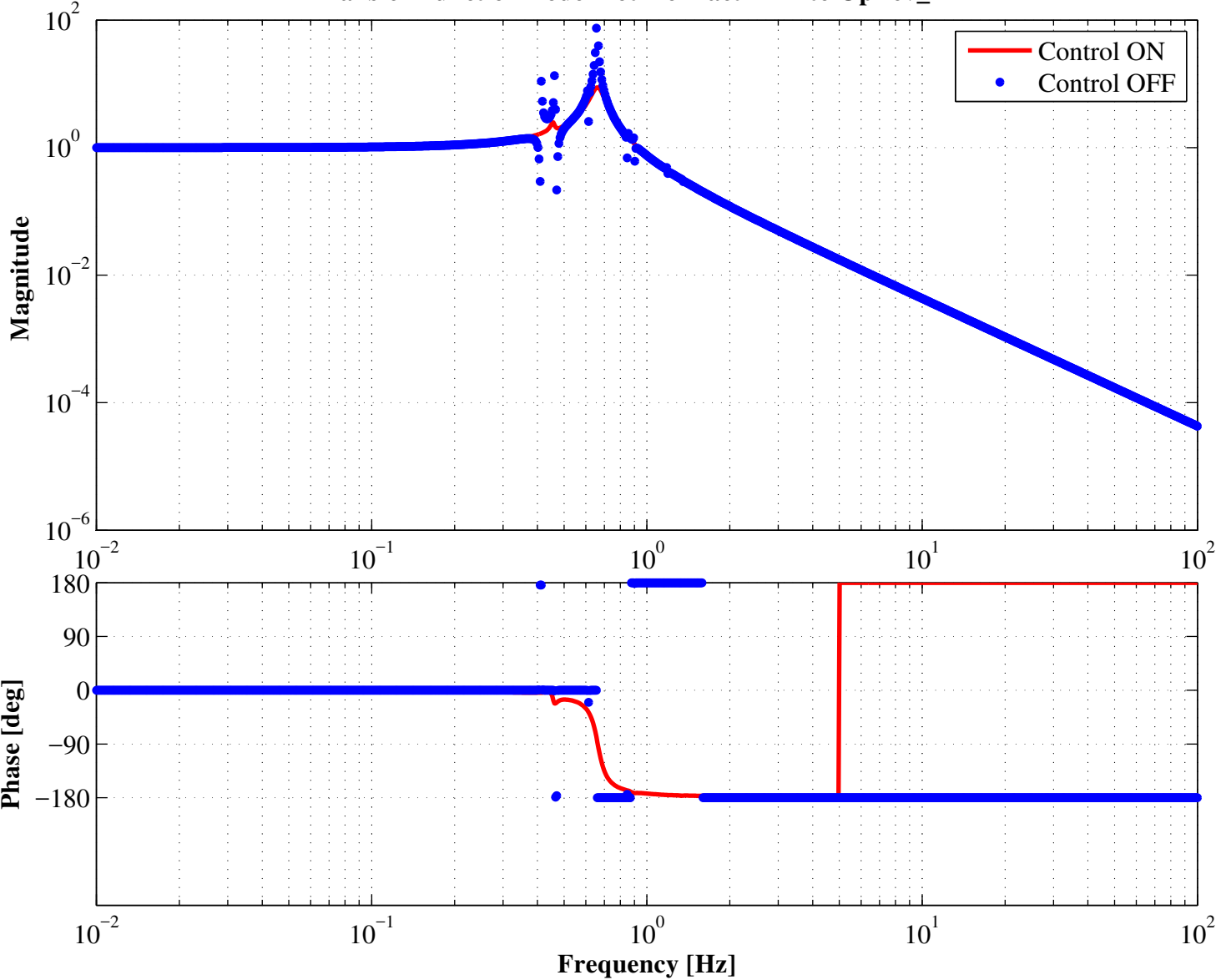
Transfer Function Bode Plot from actLTM to OpLev_LTM
