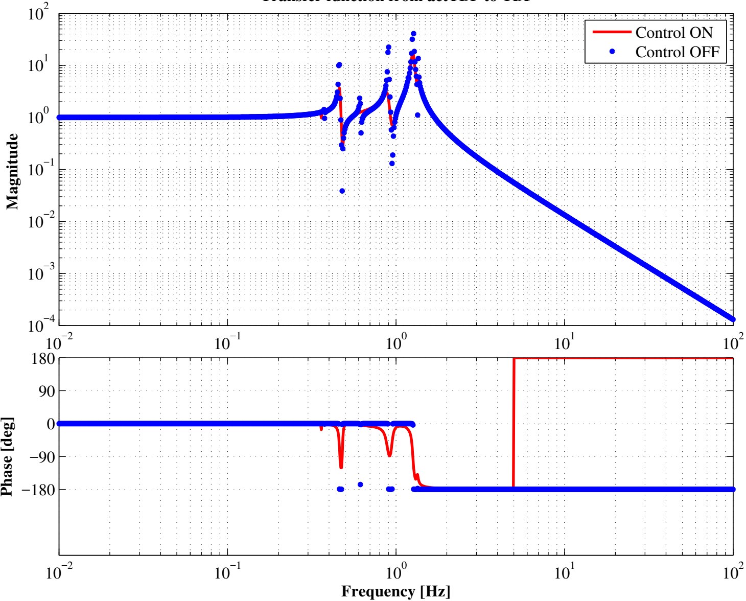
Transfer function from actTBF to TBF
