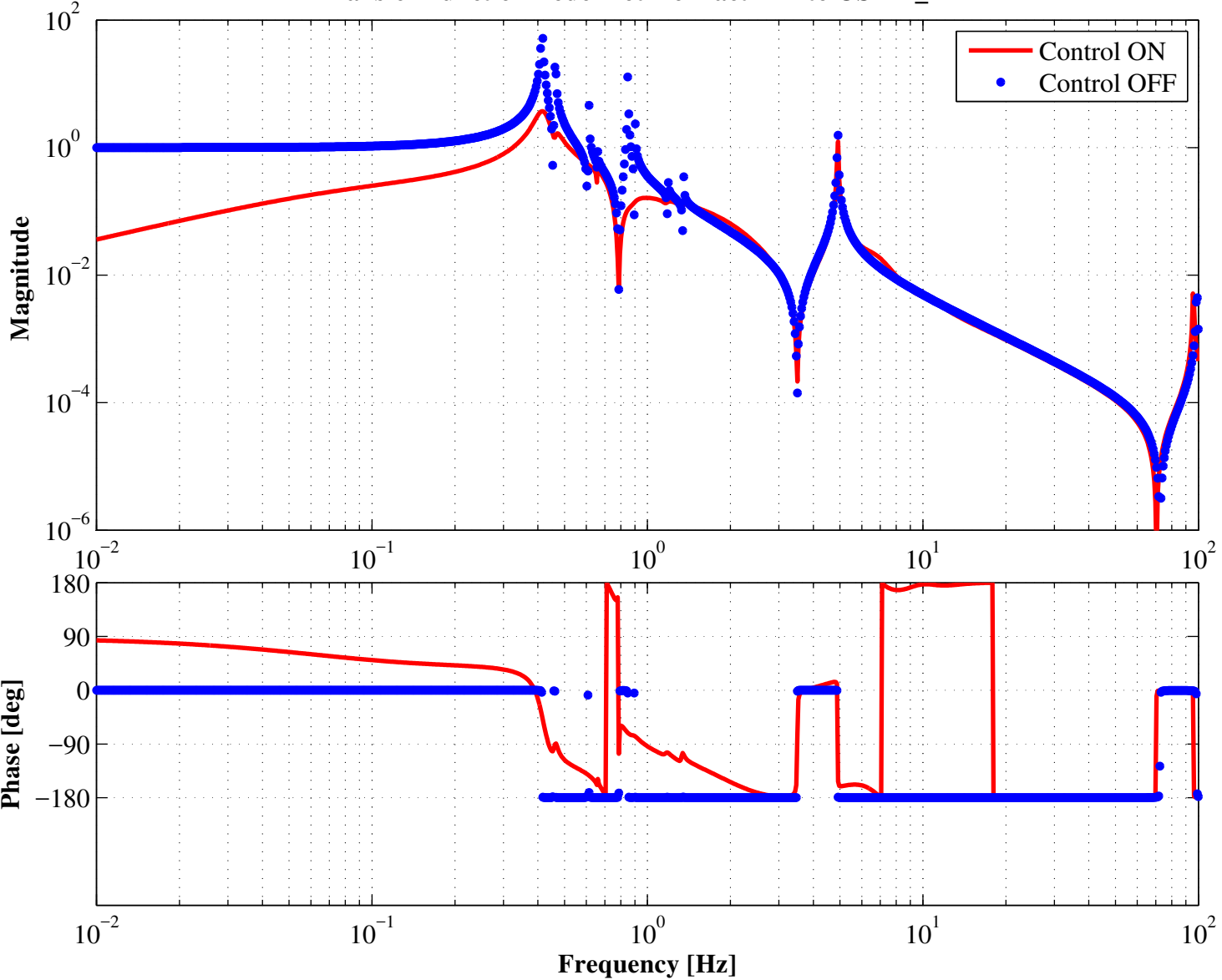
Transfer Function Bode Plot from actPIM to OSEM_PIM
