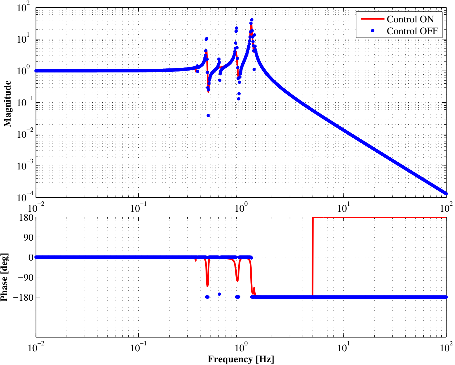
Transfer function from actTBF to TBF
