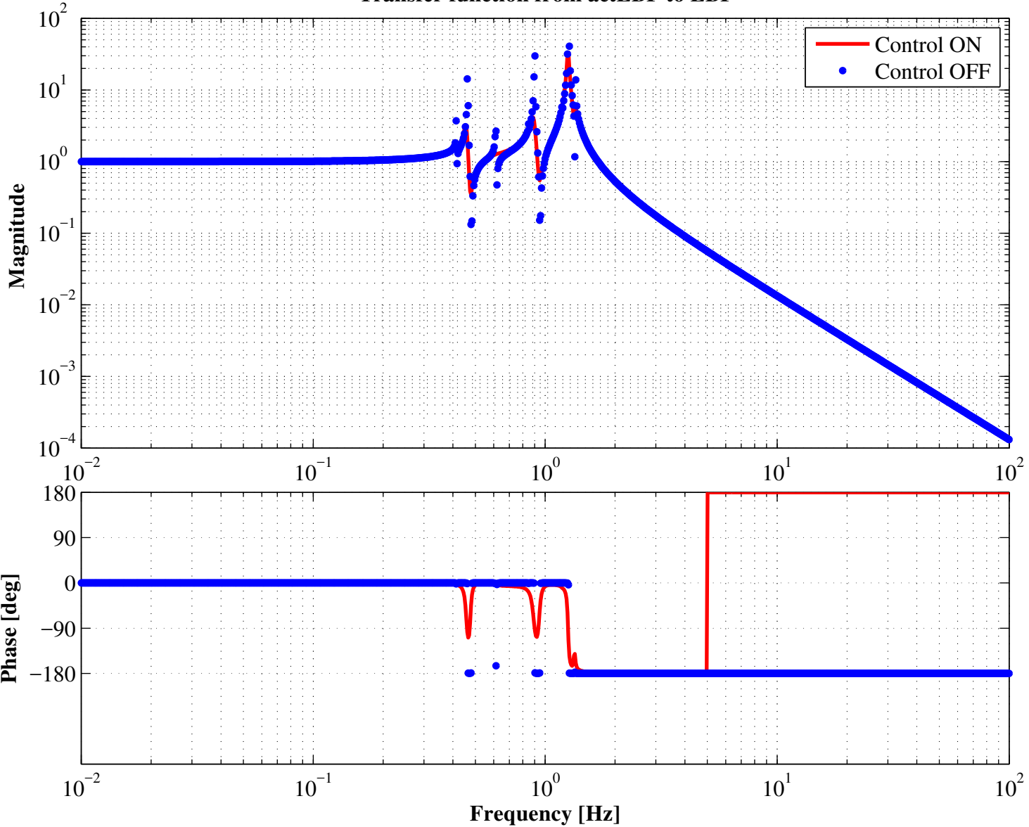
Transfer function from actLBF to LBF
