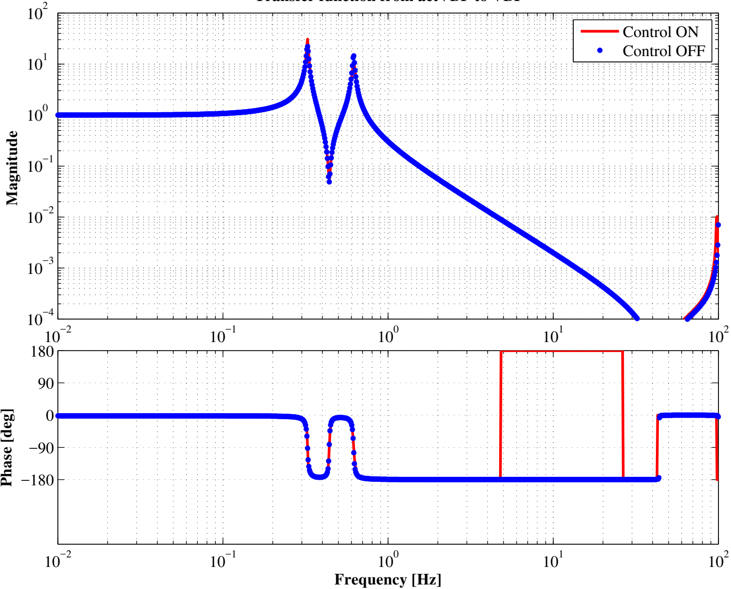
Transfer function from actVBF to VBF
