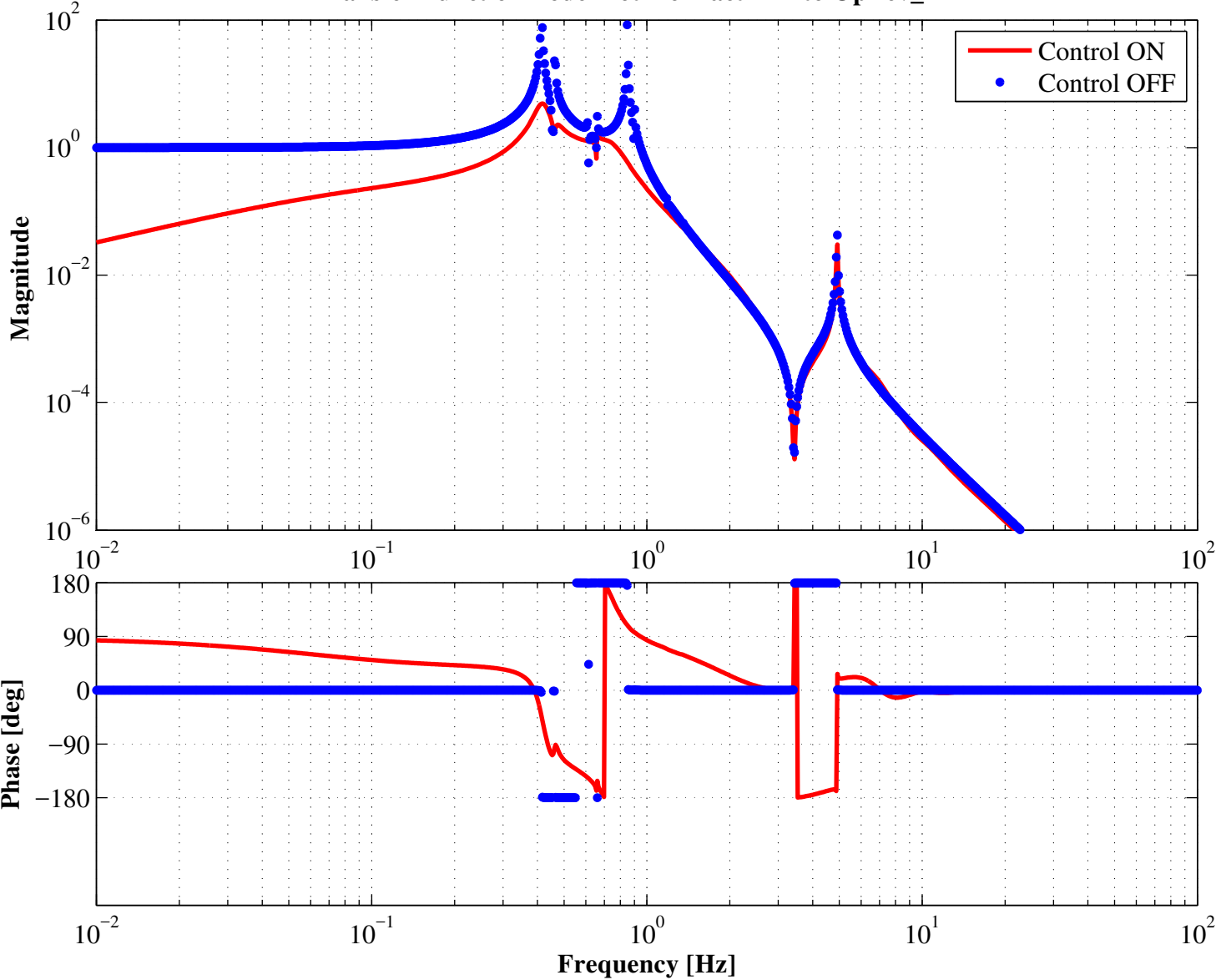
Transfer Function Bode Plot from actPIM to OpLev_PTM
