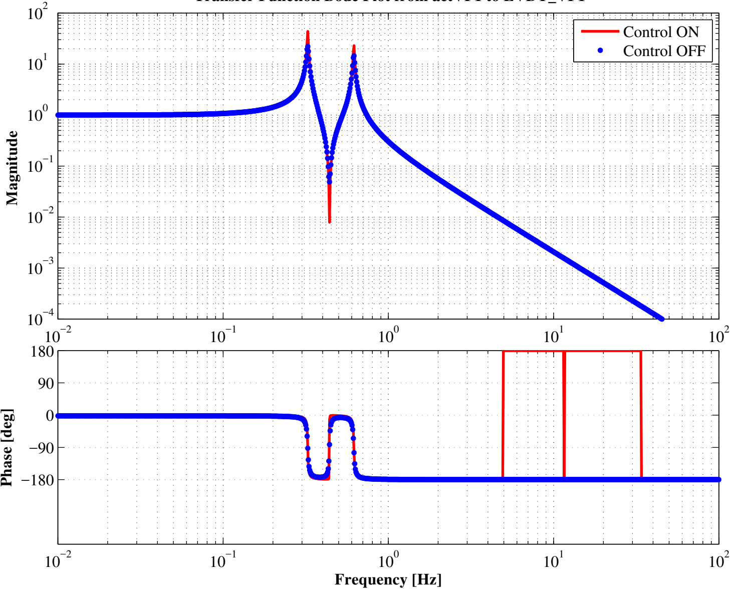
Transfer Function Bode Plot from actVF1 to LVDT_VF1
