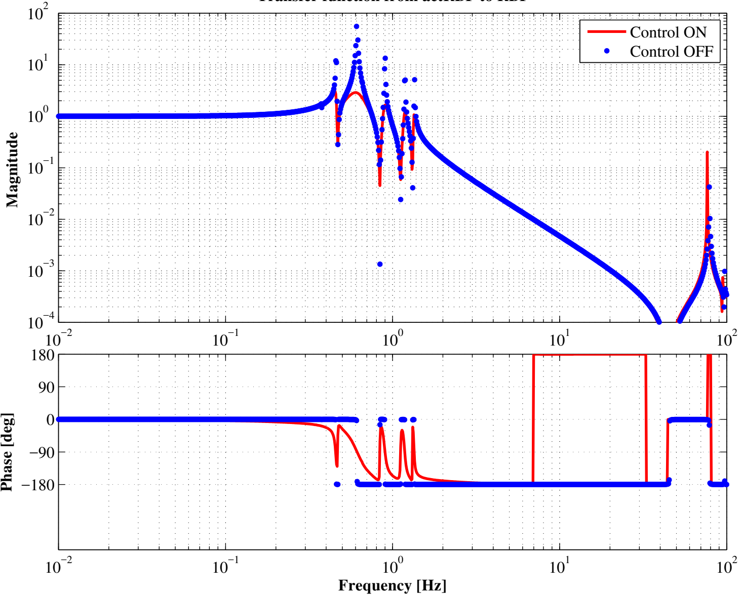
Transfer function from actRBF to RBF
