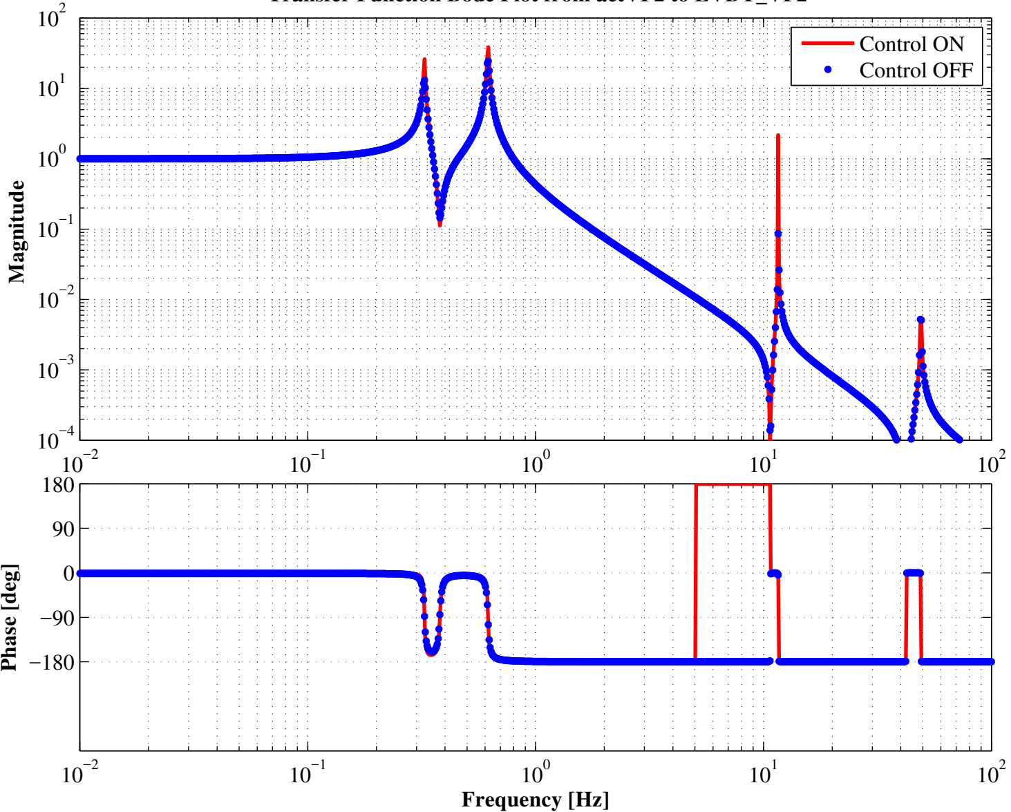
Transfer Function Bode Plot from actVF2 to LVDT_VF2
