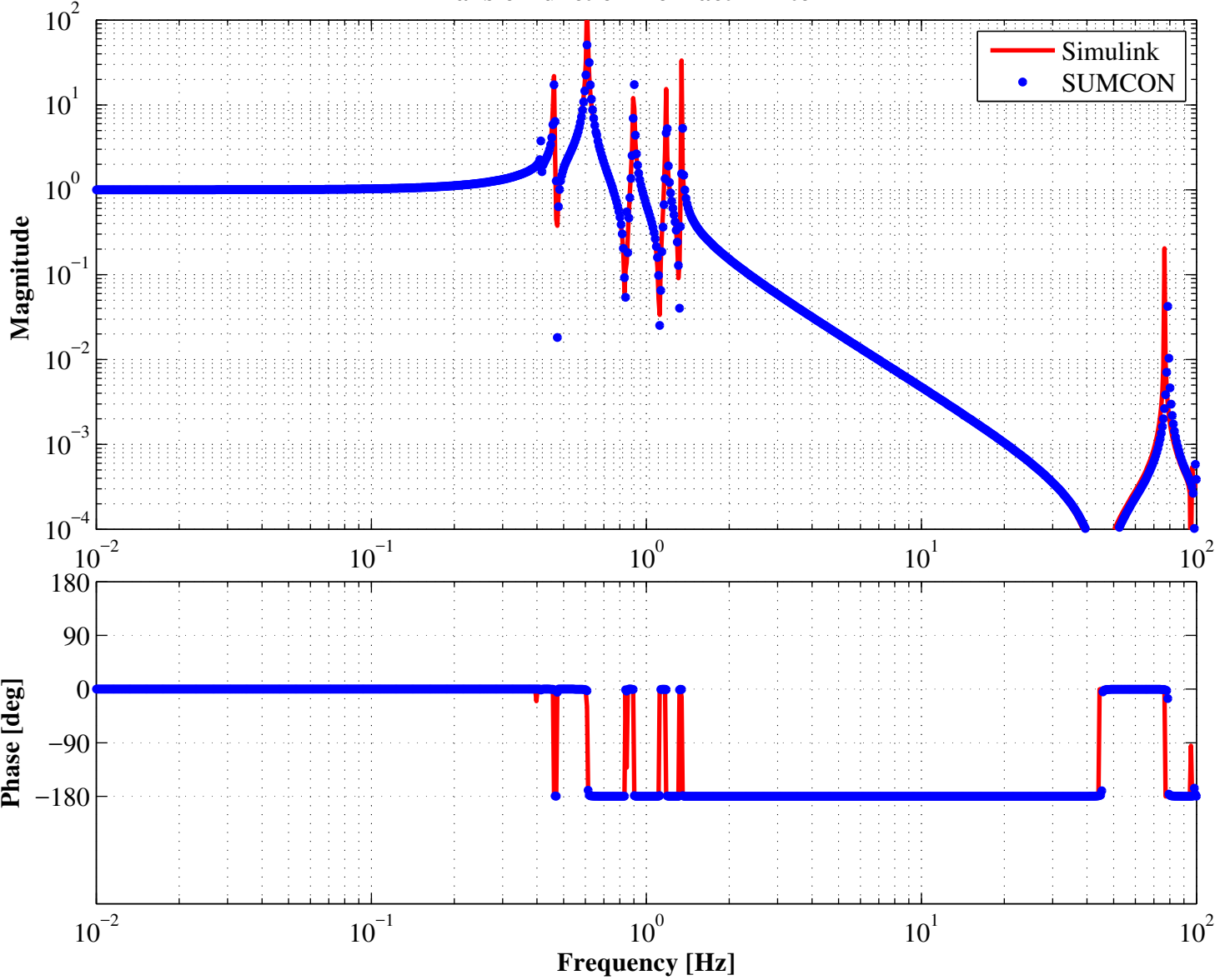
Transfer function from actPBF to PBF
