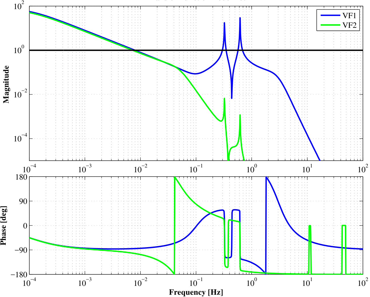
Transfer Function Bode Plot
