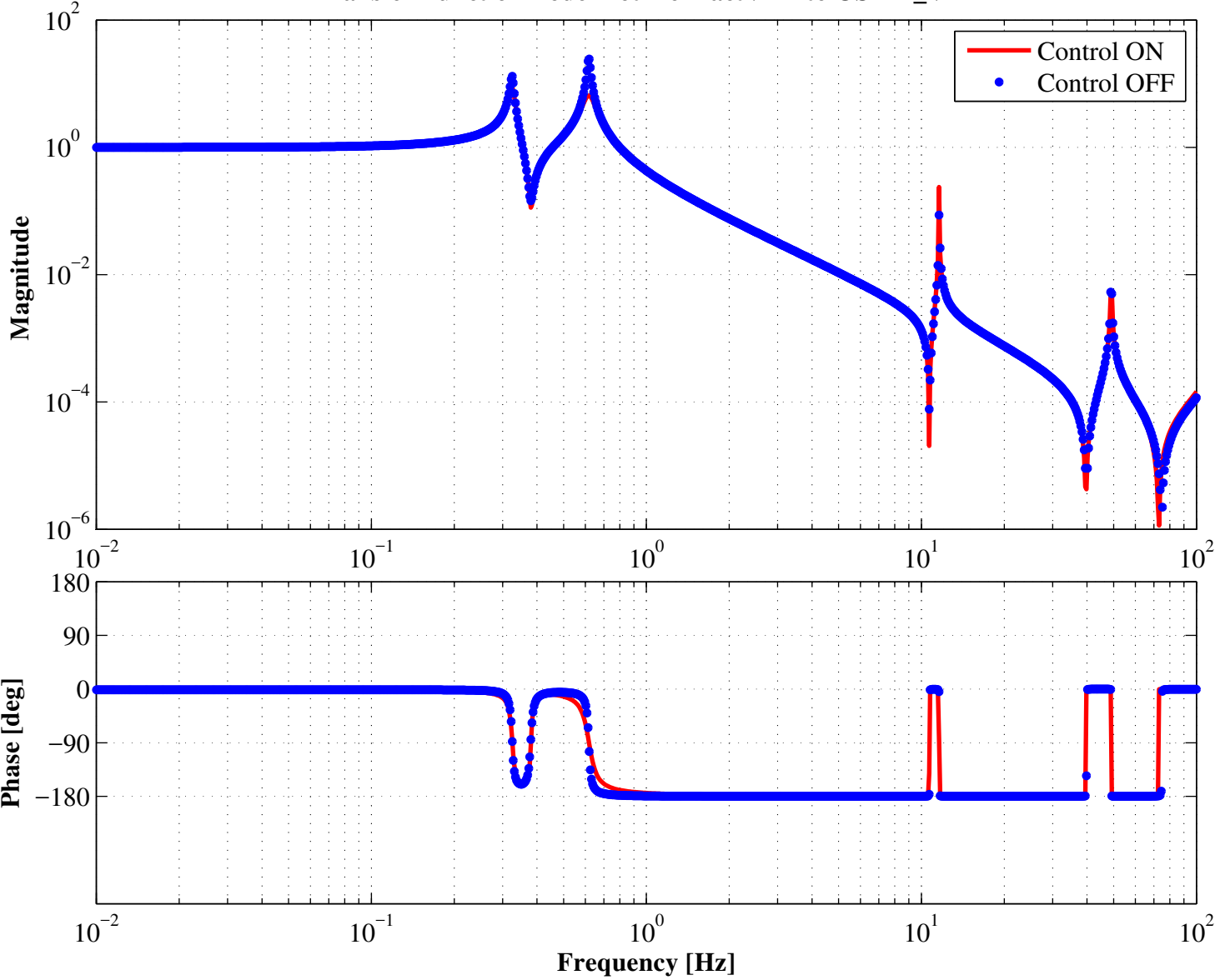
Transfer Function Bode Plot from actVIM to OSEM_VIM
