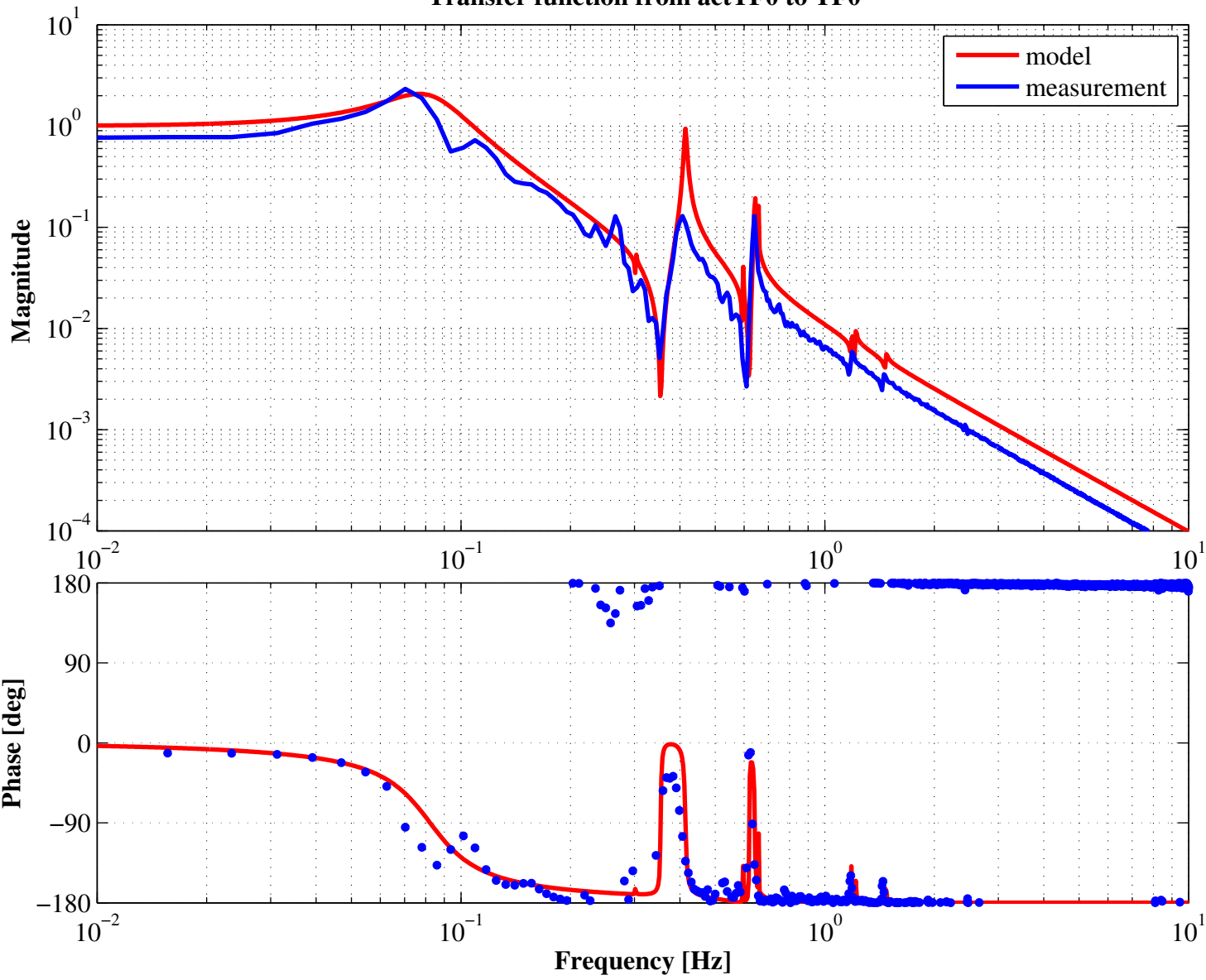
Transfer function from actTF0 to TF0
