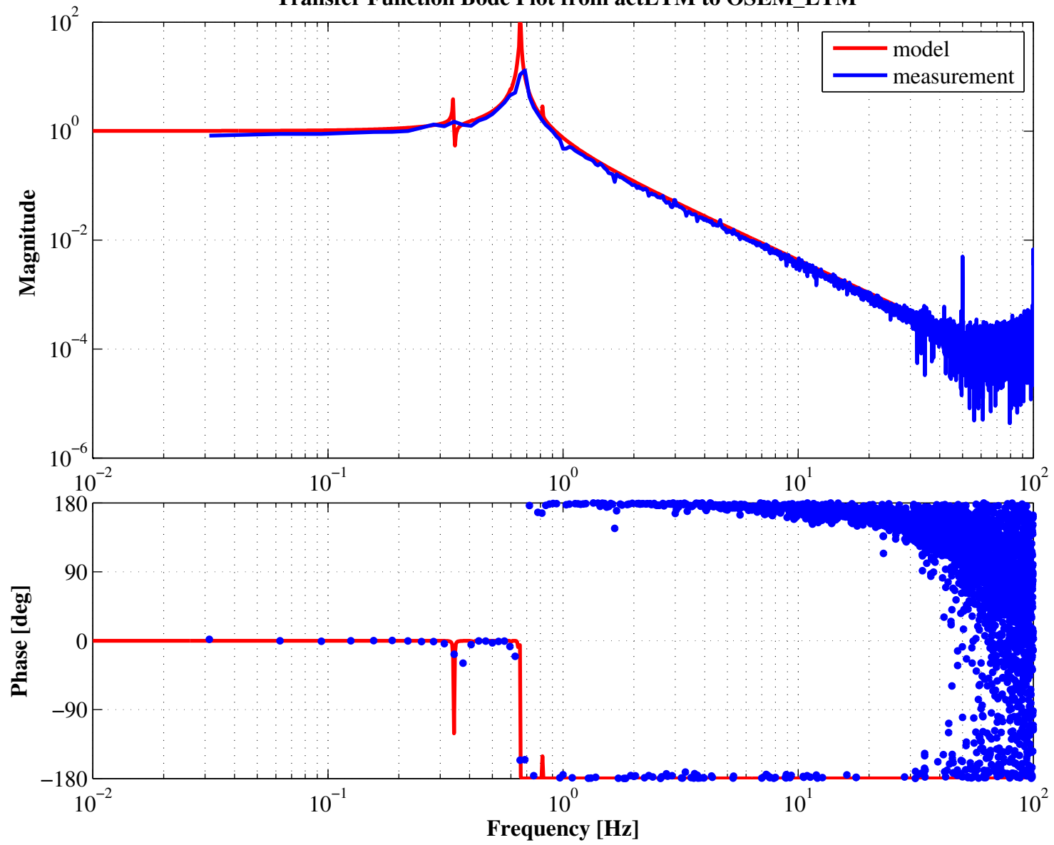
Transfer Function Bode Plot from actLTM to OSEM_LTM
