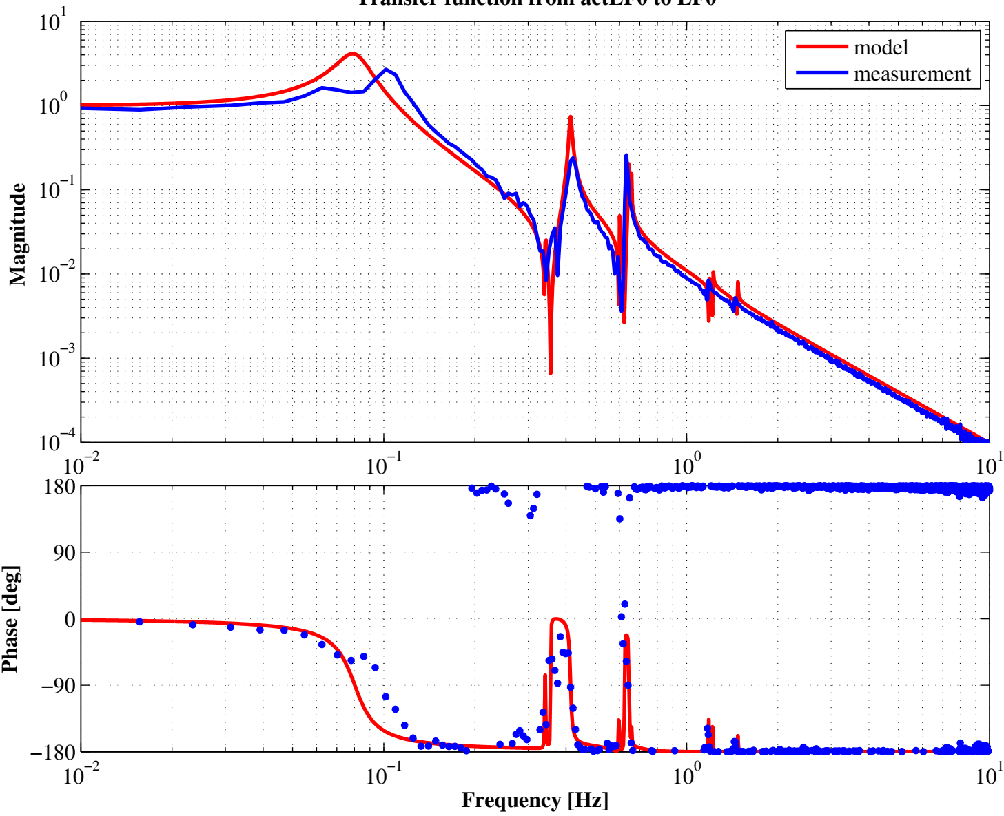
Transfer function from actLF0 to LF0
