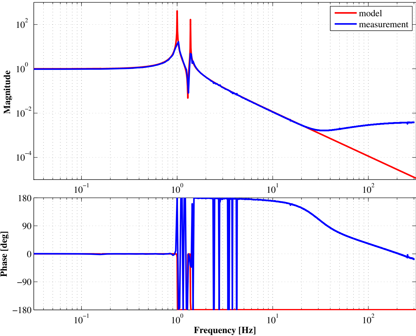
Transfer function from YTM actuator to YTM sensor
