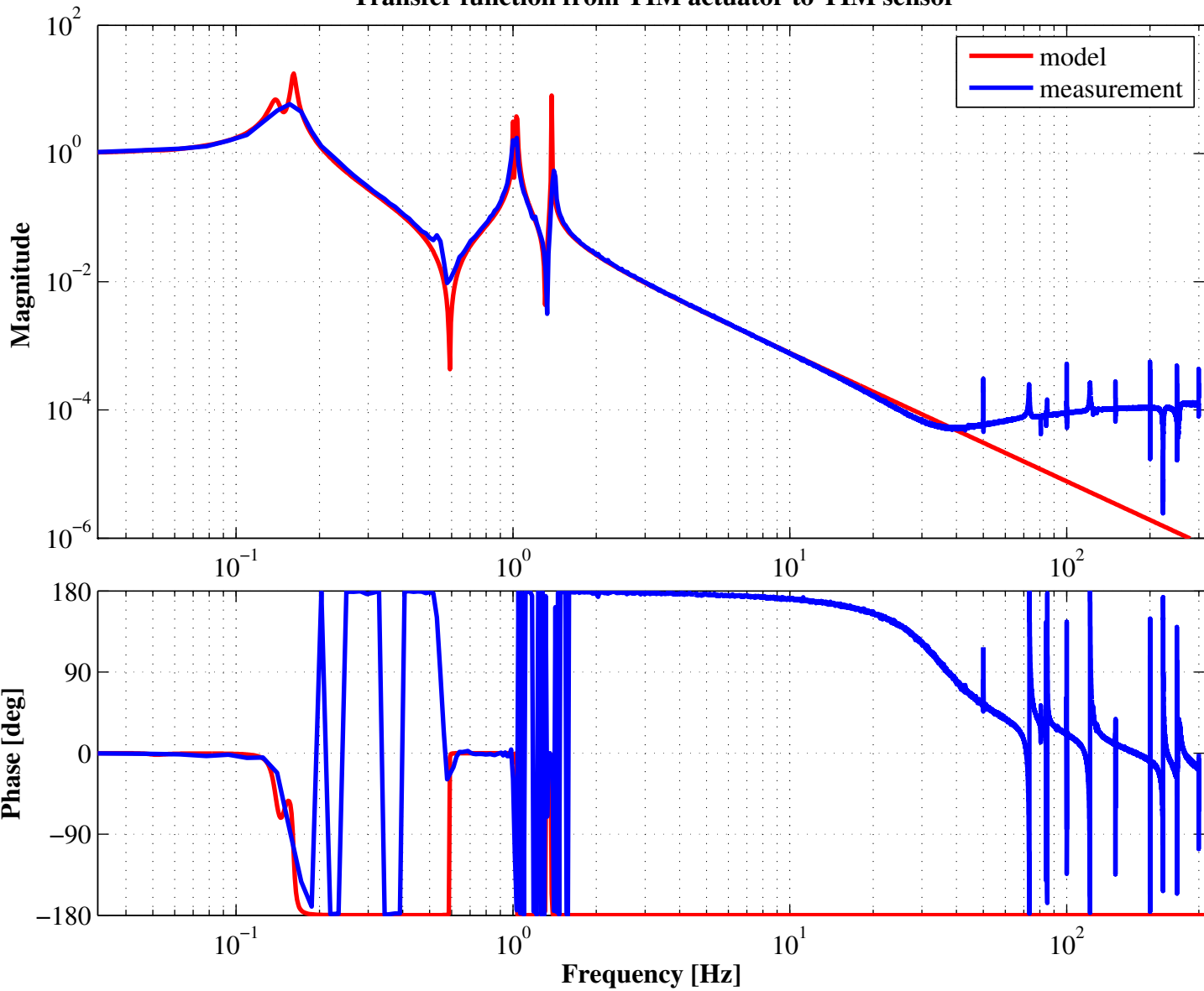
Transfer function from YIM actuator to YIM sensor
