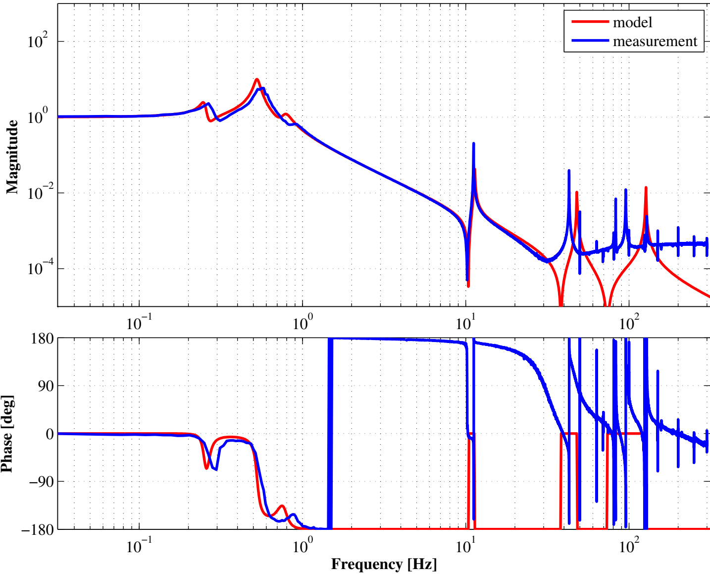
Transfer function from VIM actuator to VIM sensor
