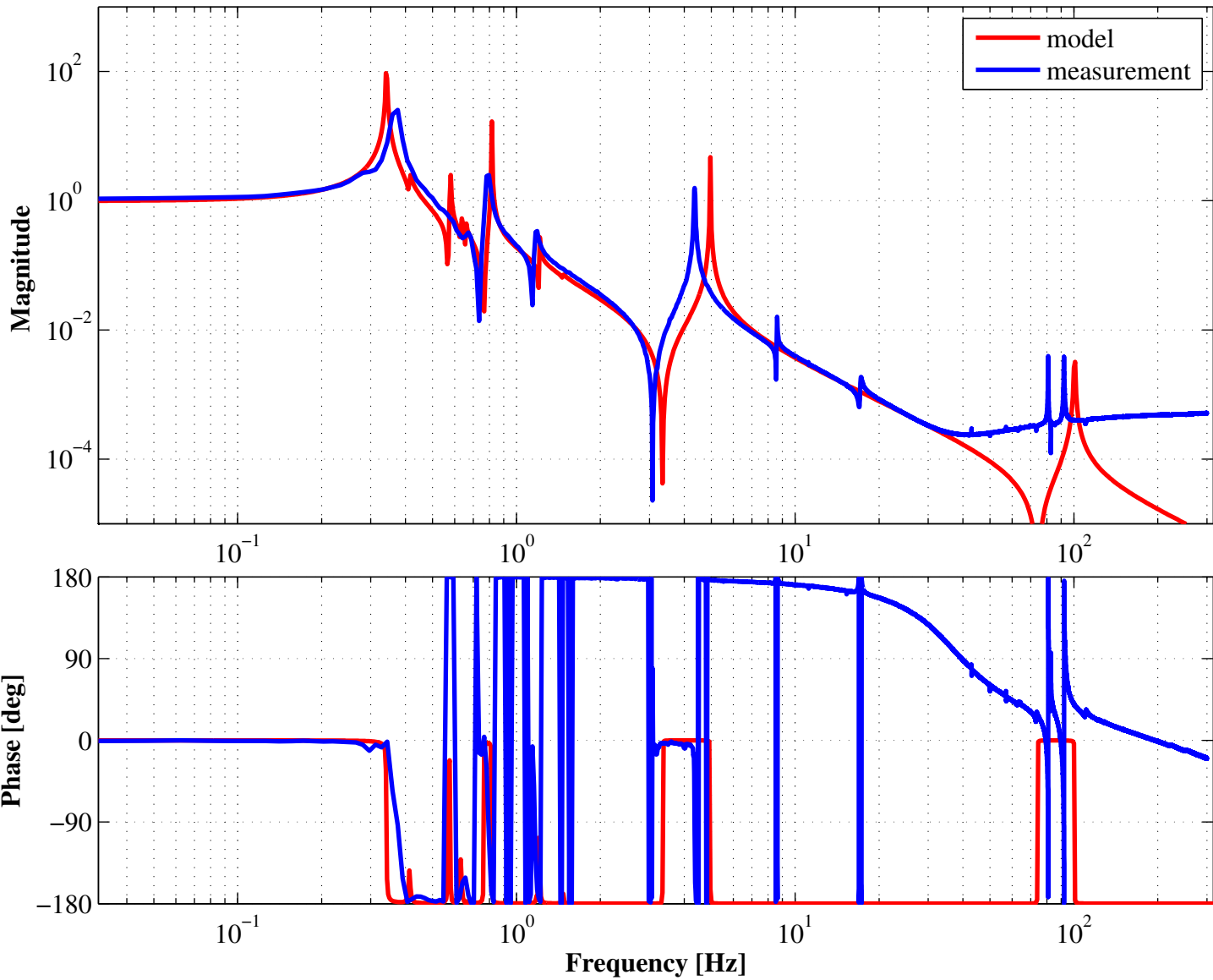
Transfer function from PIM actuator to PIM sensor
