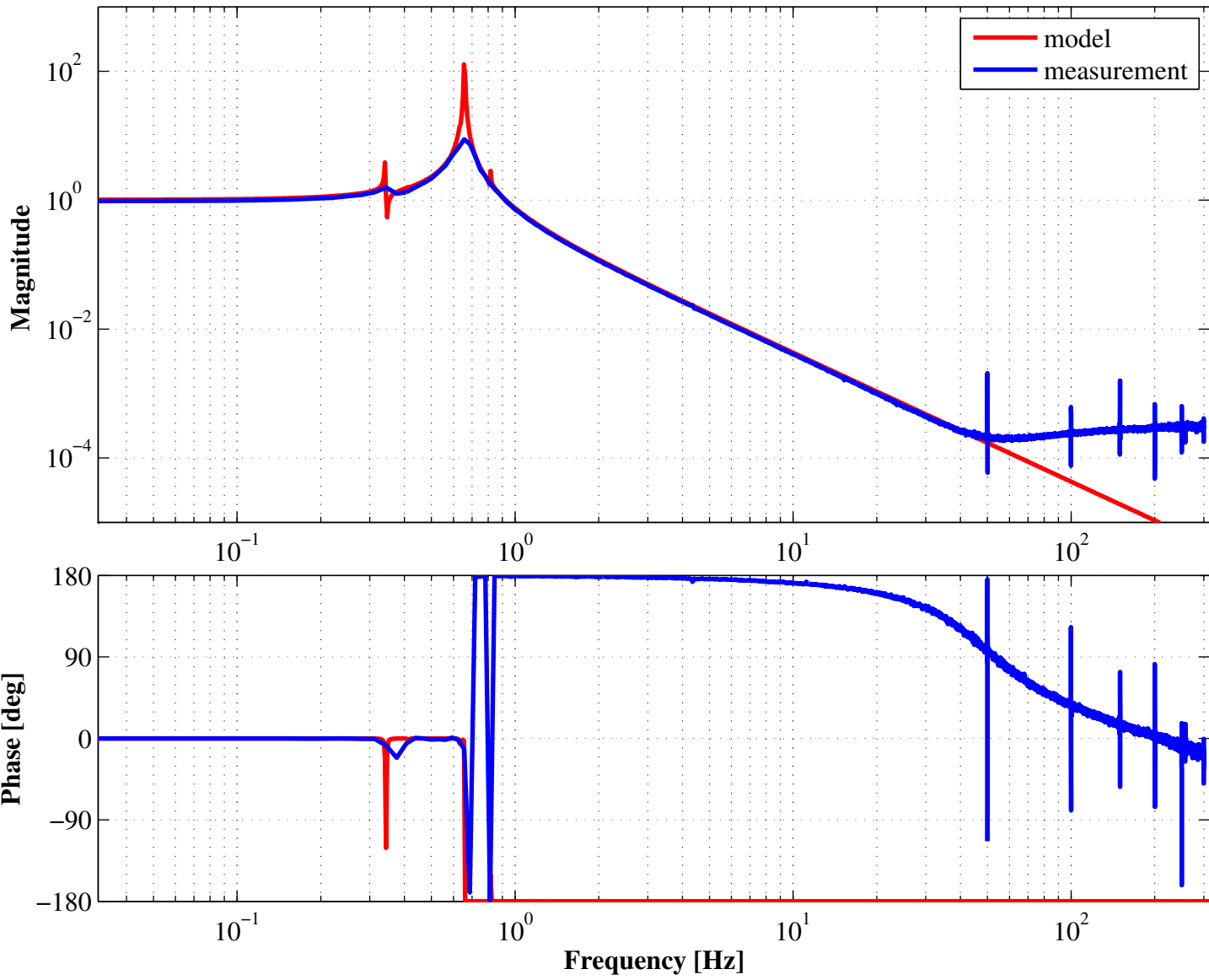
Transfer function from LTM actuator to LTM sensor
