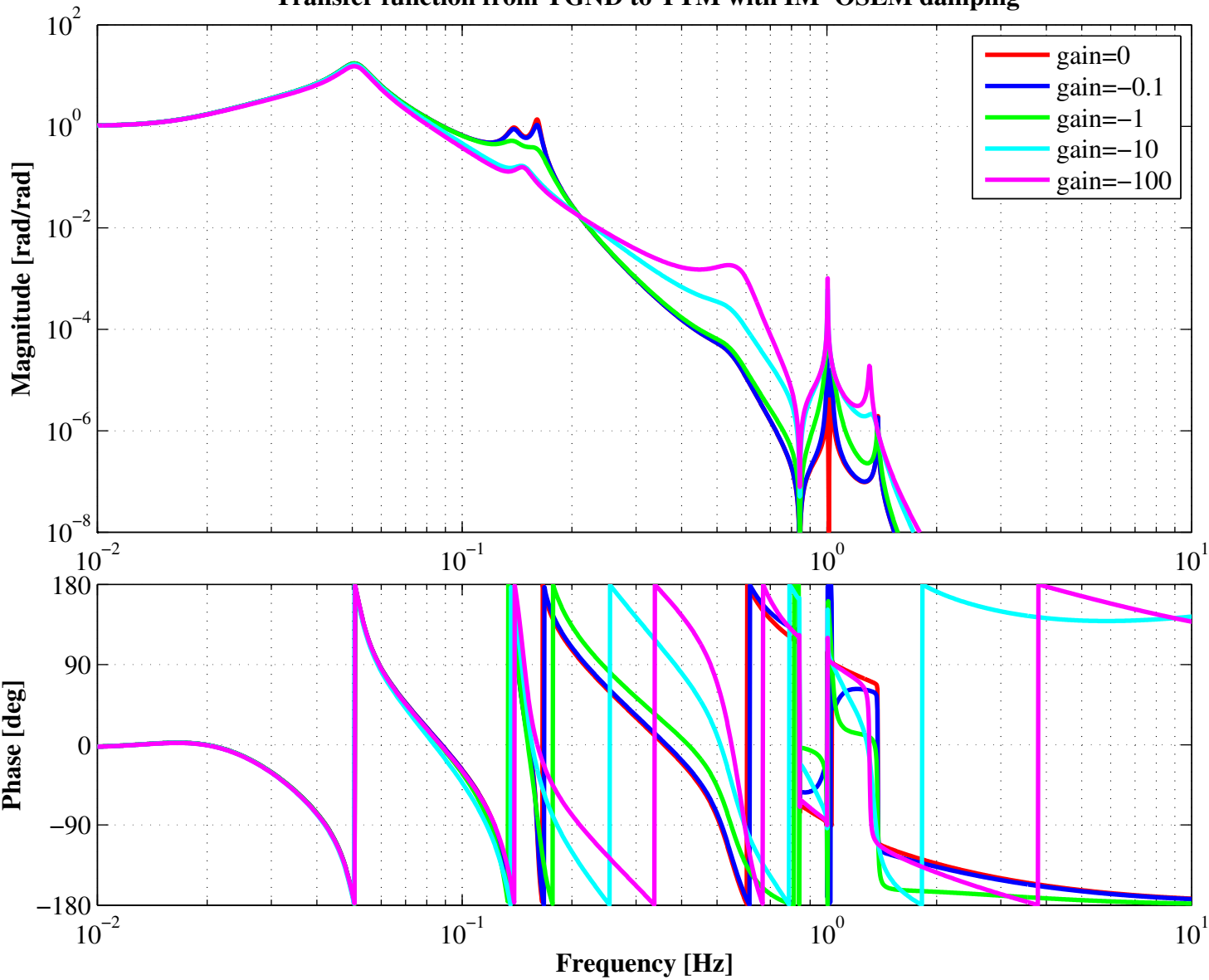
Transfer function from YGND to YTM with IM-OSEM damping
